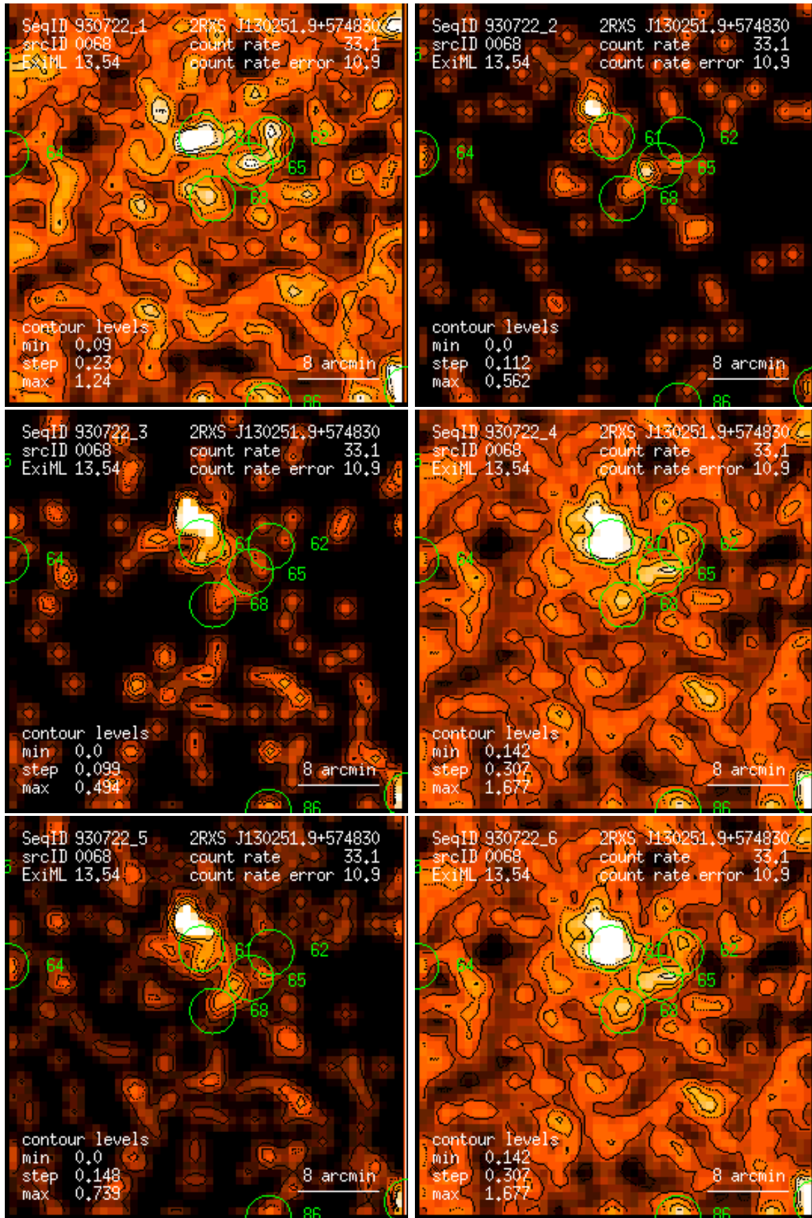
Figure 68: RASS 930722: detection 0068: band rate images, Gaussian filter: (1) PSPC channels 11 – 41, (2) 52 – 90, (3) 91 – 201, (4) 11 – 235, (5) 52 – 201, (6) 11 – 201. Broad band rates in counts/ks. Band rate contour levels in counts/ks/arcmin 2 .
