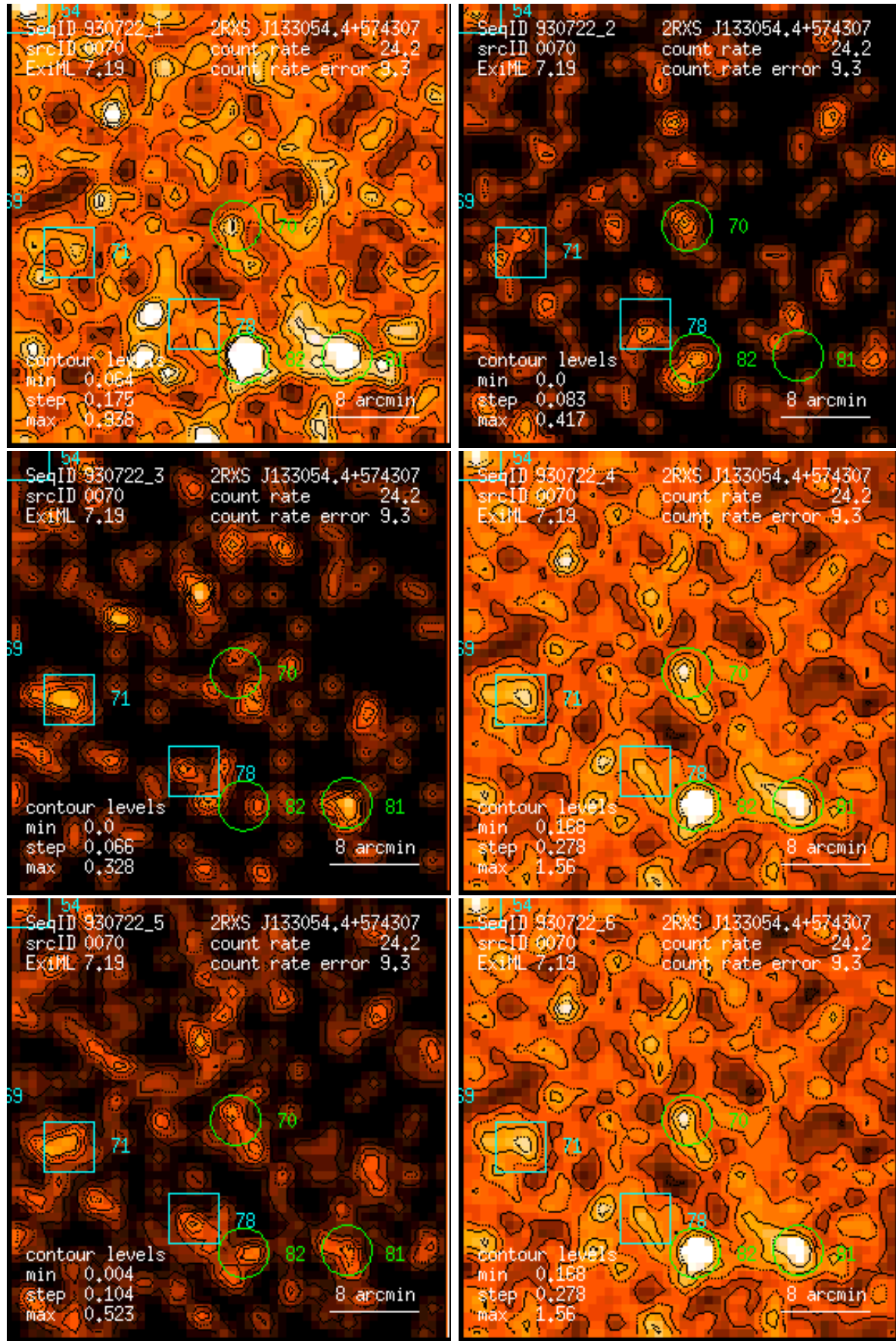
Figure 70: RASS 930722: detection 0070: band rate images, Gaussian filter: (1) PSPC channels 11 – 41, (2) 52 – 90, (3) 91 – 201, (4) 11 – 235, (5) 52 – 201, (6) 11 – 201. Broad band rates in counts/ks. Band rate contour levels in counts/ks/arcmin 2 .
