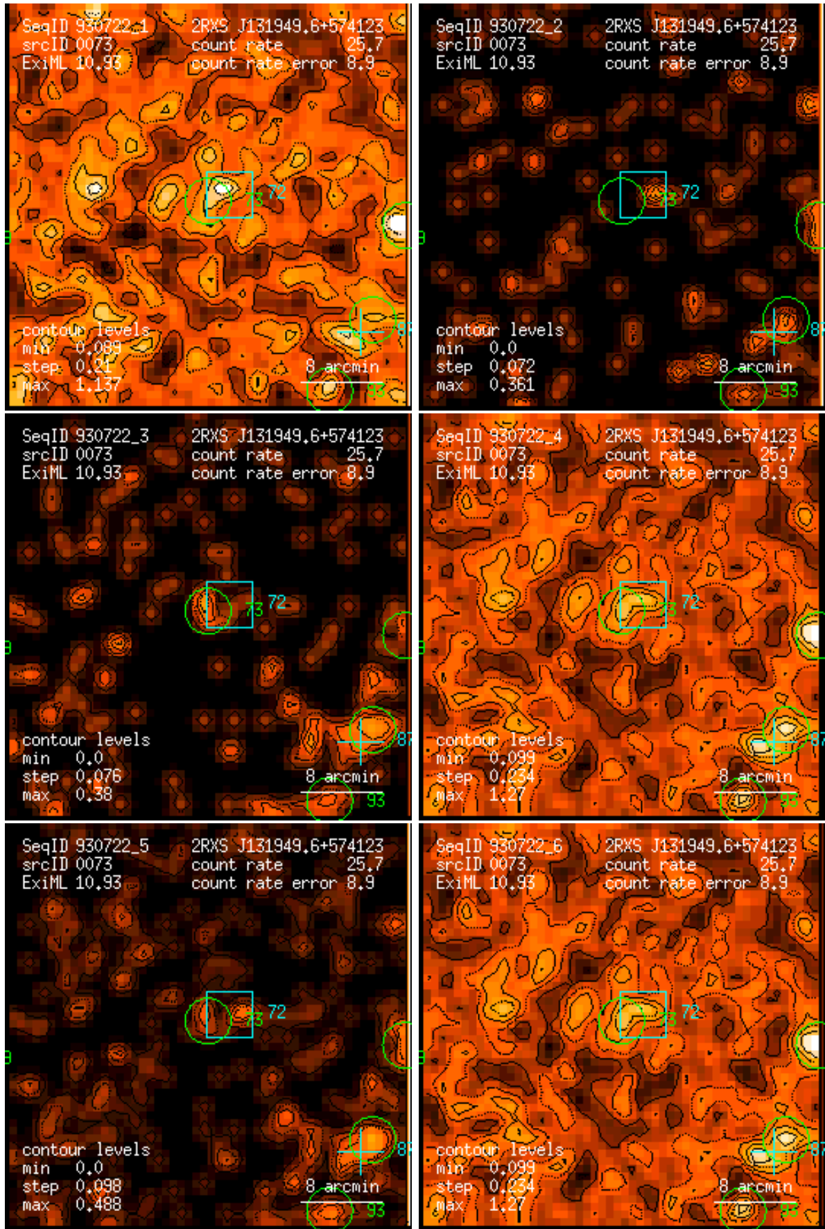
Figure 73: RASS 930722: detection 0073: band rate images, Gaussian filter: (1) PSPC channels 11 – 41, (2) 52 – 90, (3) 91 – 201, (4) 11 – 235, (5) 52 – 201, (6) 11 – 201. Broad band rates in counts/ks. Band rate contour levels in counts/ks/arcmin 2 .
