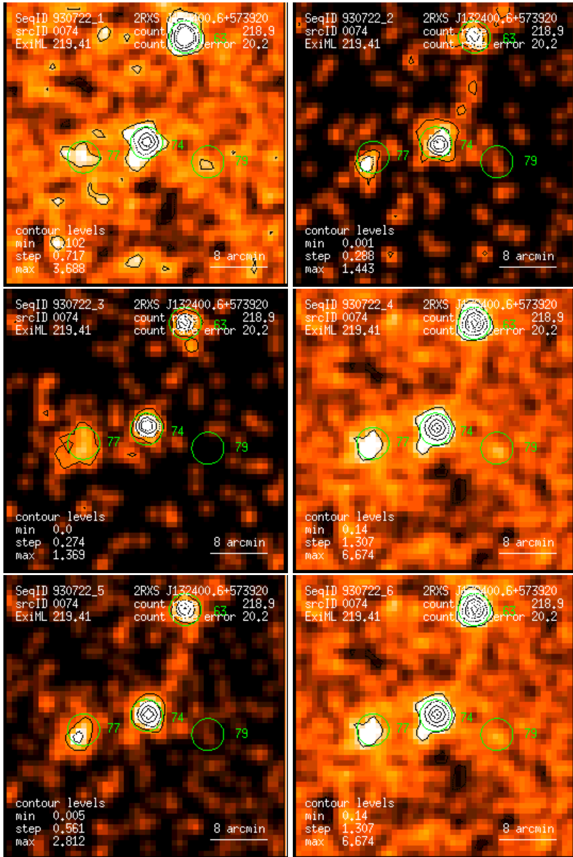
Figure 74: RASS 930722: detection 0074: band rate images, Gaussian filter: (1) PSPC channels 11 – 41, (2) 52 – 90, (3) 91 – 201, (4) 11 – 235, (5) 52 – 201, (6) 11 – 201. Broad band rates in counts/ks. Band rate contour levels in counts/ks/arcmin 2 .
