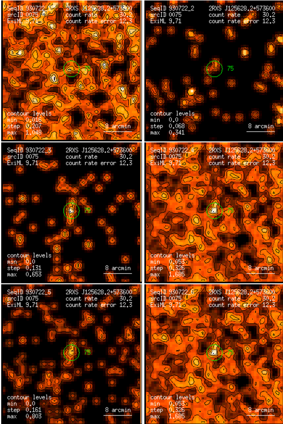
Figure 75: RASS 930722: detection 0075: band rate images, Gaussian filter: (1) PSPC channels 11 – 41, (2) 52 – 90, (3) 91 – 201, (4) 11 – 235, (5) 52 – 201, (6) 11 – 201. Broad band rates in counts/ks. Band rate contour levels in counts/ks/arcmin 2 .
