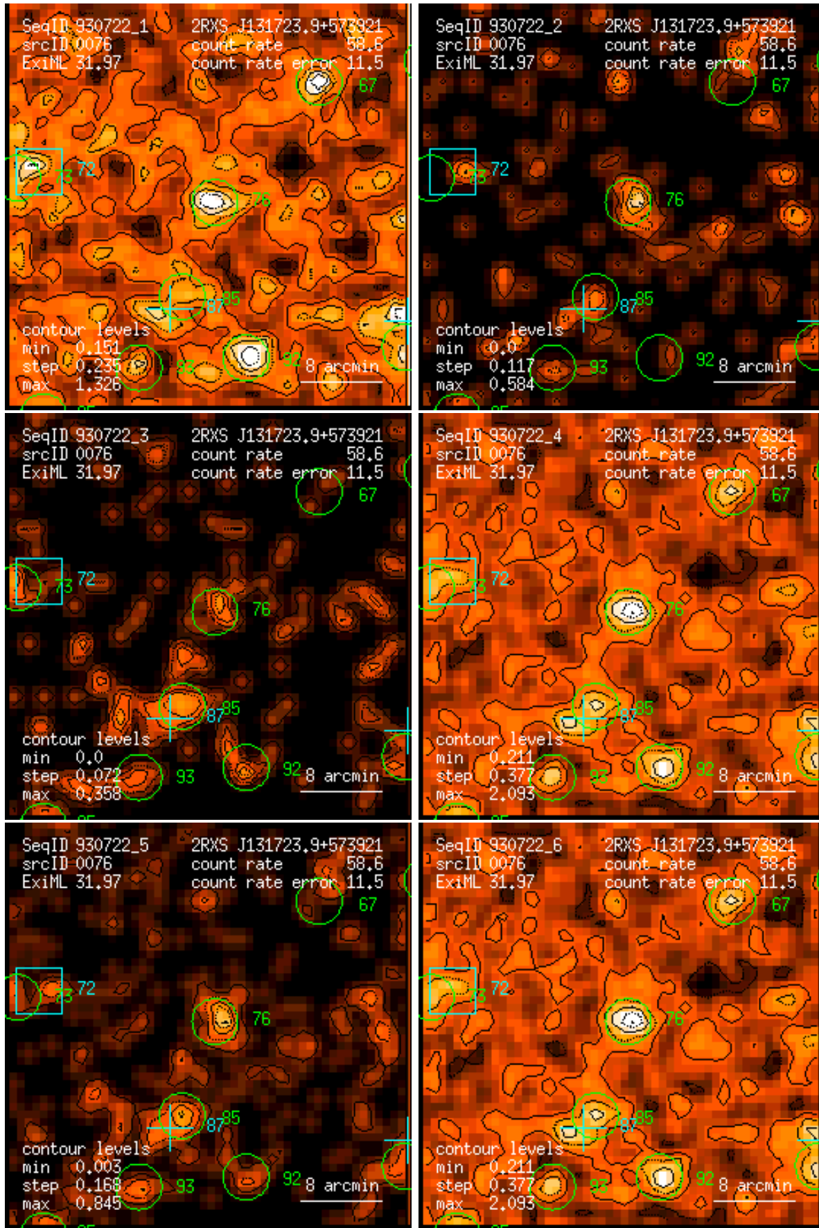
Figure 76: RASS 930722: detection 0076: band rate images, Gaussian filter: (1) PSPC channels 11 – 41, (2) 52 – 90, (3) 91 – 201, (4) 11 – 235, (5) 52 – 201, (6) 11 – 201. Broad band rates in counts/ks. Band rate contour levels in counts/ks/arcmin 2 .
