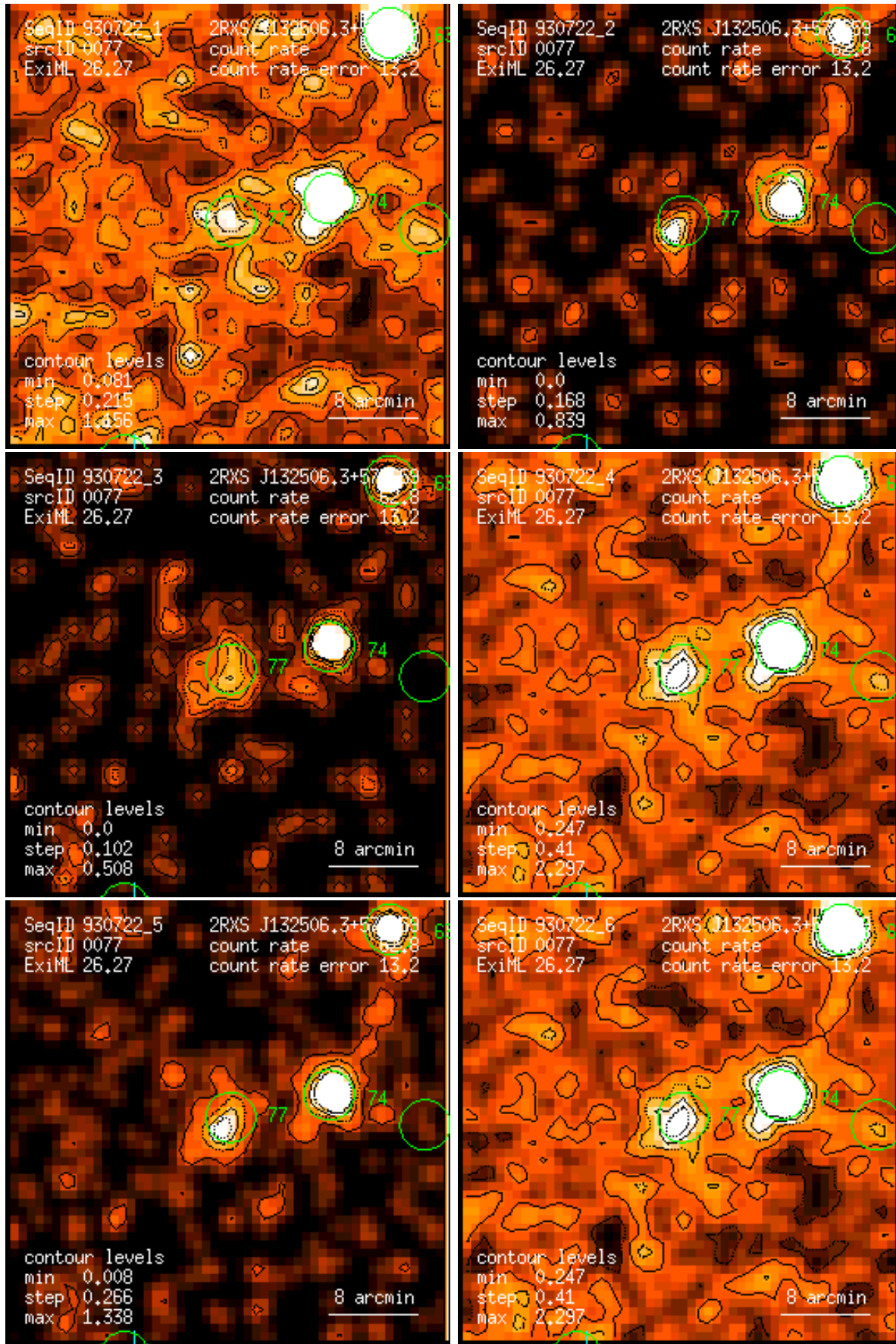
Figure 77: RASS 930722: detection 0077: band rate images, Gaussian filter: (1) PSPC channels 11 – 41, (2) 52 – 90, (3) 91 – 201, (4) 11 – 235, (5) 52 – 201, (6) 11 – 201. Broad band rates in counts/ks. Band rate contour levels in counts/ks/arcmin 2 .
