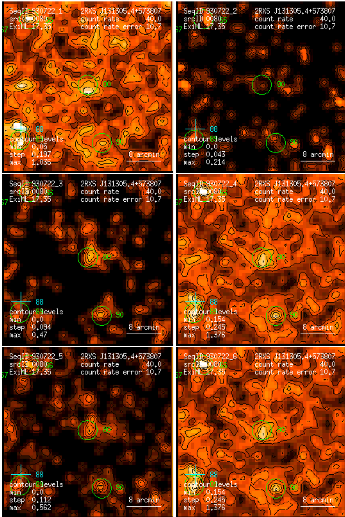
Figure 80: RASS 930722: detection 0080: band rate images, Gaussian filter: (1) PSPC channels 11 – 41, (2) 52 – 90, (3) 91 – 201, (4) 11 – 235, (5) 52 – 201, (6) 11 – 201. Broad band rates in counts/ks. Band rate contour levels in counts/ks/arcmin 2 .
