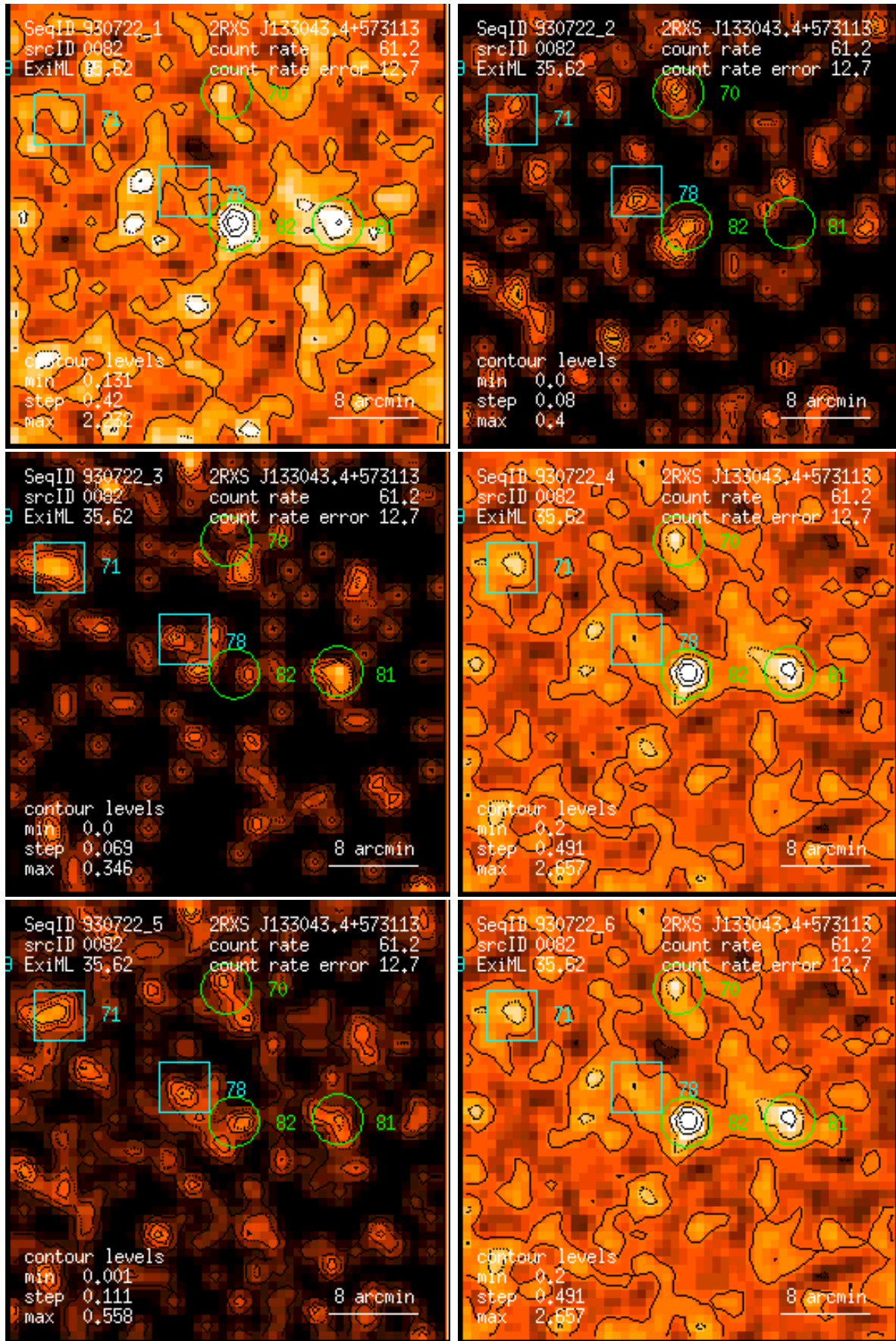
Figure 82: RASS 930722: detection 0082: band rate images, Gaussian filter: (1) PSPC channels 11 – 41, (2) 52 – 90, (3) 91 – 201, (4) 11 – 235, (5) 52 – 201, (6) 11 – 201. Broad band rates in counts/ks. Band rate contour levels in counts/ks/arcmin 2 .
