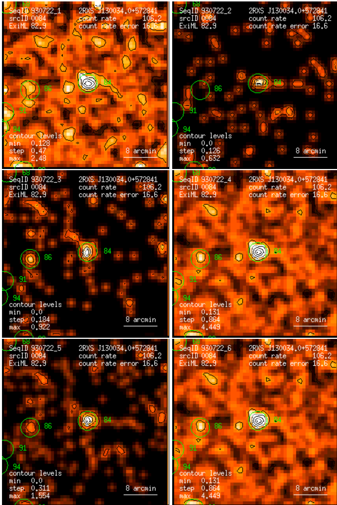
Figure 84: RASS 930722: detection 0084: band rate images, Gaussian filter: (1) PSPC channels 11 – 41, (2) 52 – 90, (3) 91 – 201, (4) 11 – 235, (5) 52 – 201, (6) 11 – 201. Broad band rates in counts/ks. Band rate contour levels in counts/ks/arcmin 2 .
