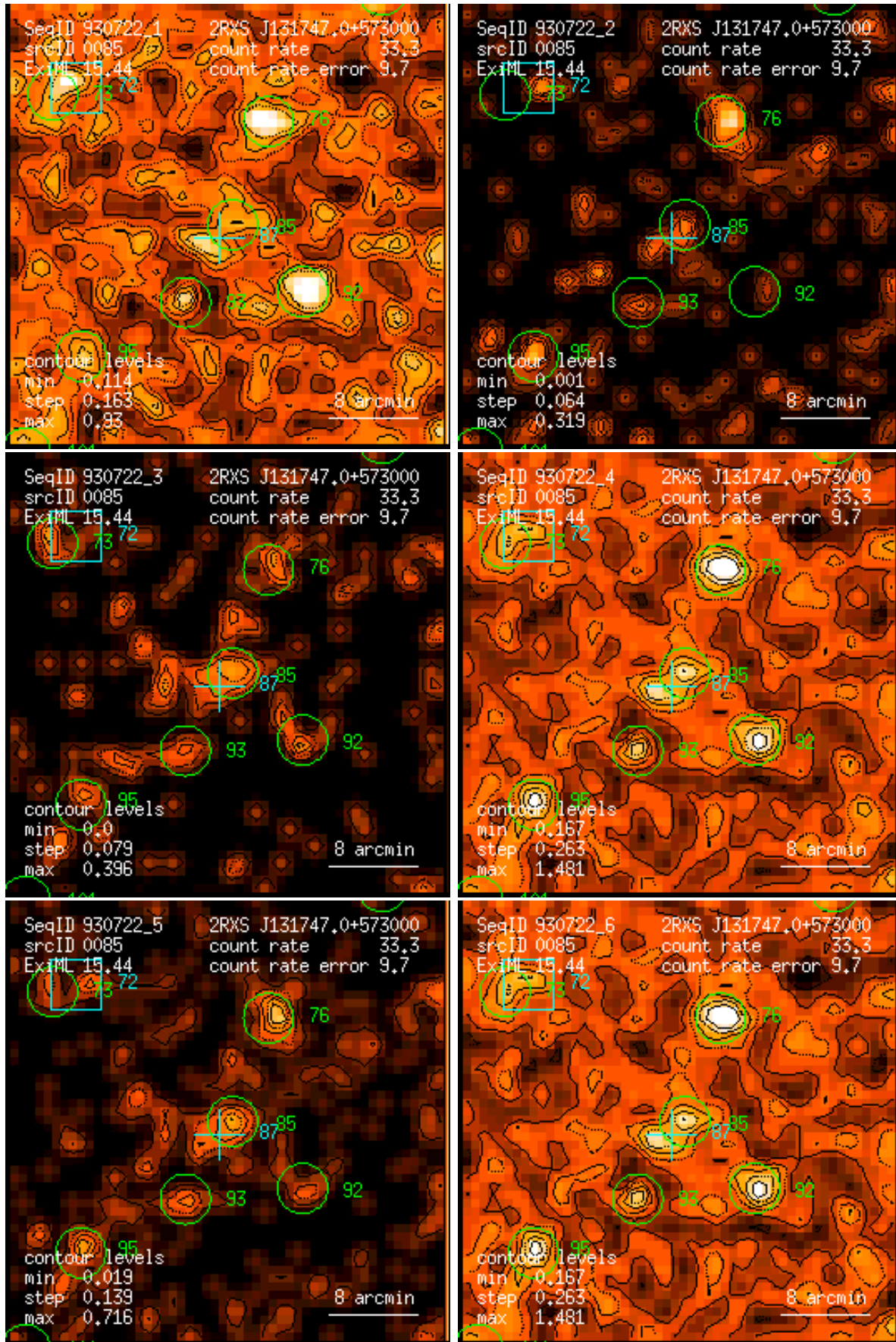
Figure 85: RASS 930722: detection 0085: band rate images, Gaussian filter: (1) PSPC channels 11 – 41, (2) 52 – 90, (3) 91 – 201, (4) 11 – 235, (5) 52 – 201, (6) 11 – 201. Broad band rates in counts/ks. Band rate contour levels in counts/ks/arcmin 2 .
