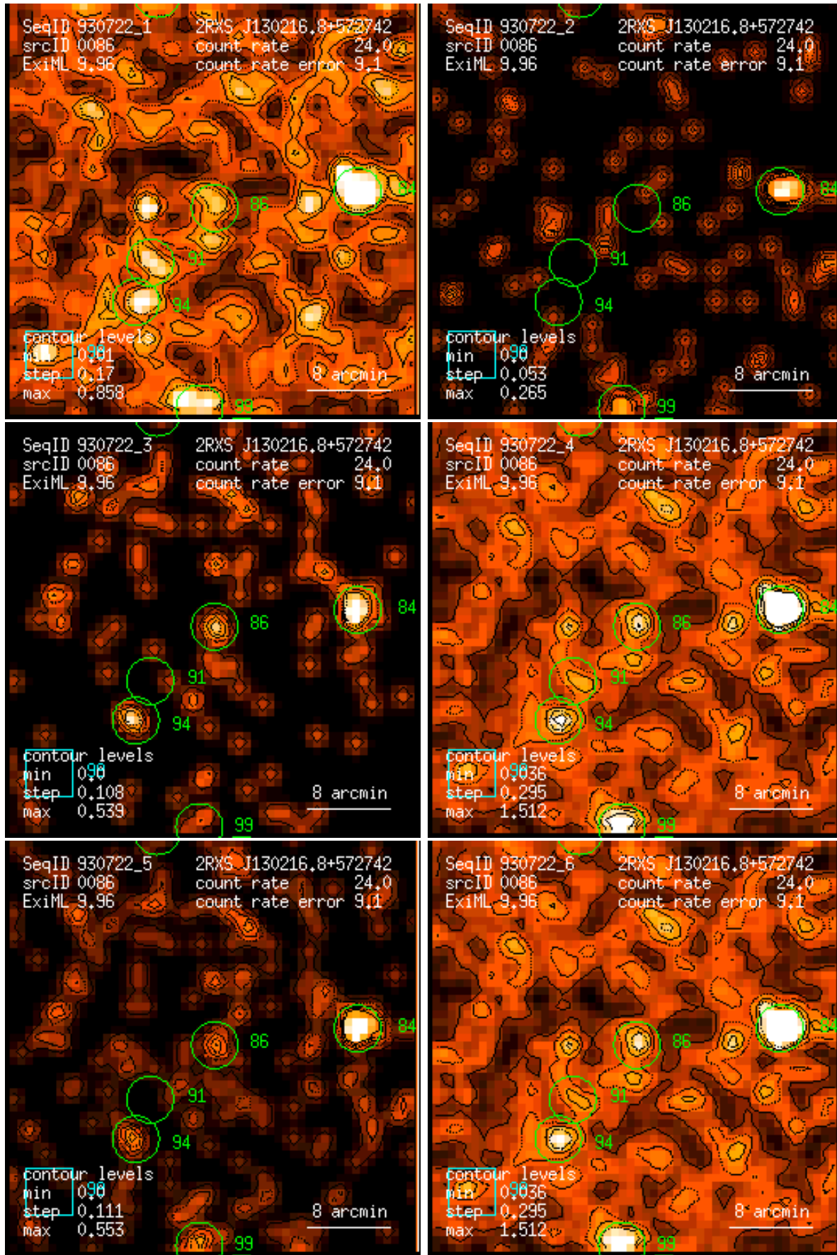
Figure 86: RASS 930722: detection 0086: band rate images, Gaussian filter: (1) PSPC channels 11 – 41, (2) 52 – 90, (3) 91 – 201, (4) 11 – 235, (5) 52 – 201, (6) 11 – 201. Broad band rates in counts/ks. Band rate contour levels in counts/ks/arcmin 2 .
