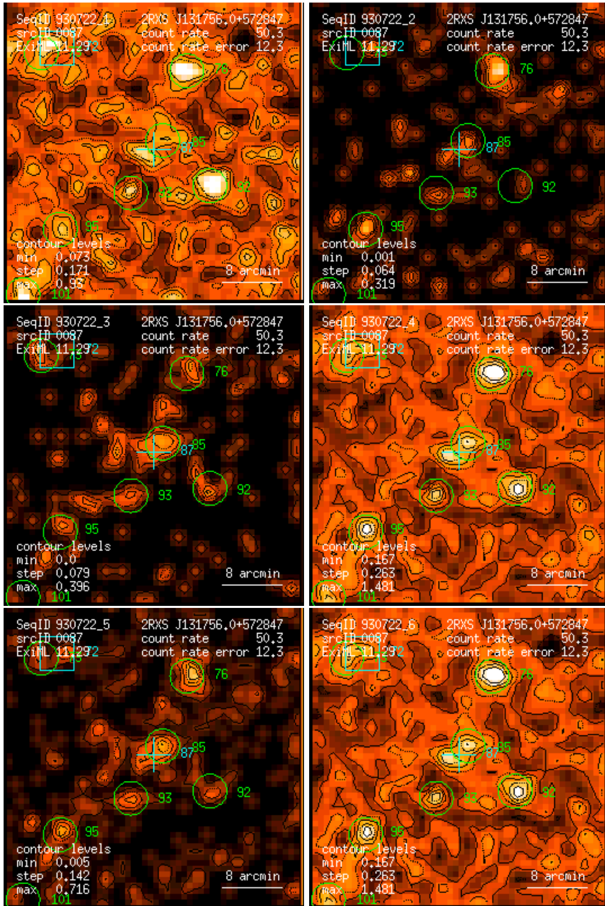
Figure 87: RASS 930722: detection 0087: band rate images, Gaussian filter: (1) PSPC channels 11 – 41, (2) 52 – 90, (3) 91 – 201, (4) 11 – 235, (5) 52 – 201, (6) 11 – 201. Broad band rates in counts/ks. Band rate contour levels in counts/ks/arcmin 2 .
