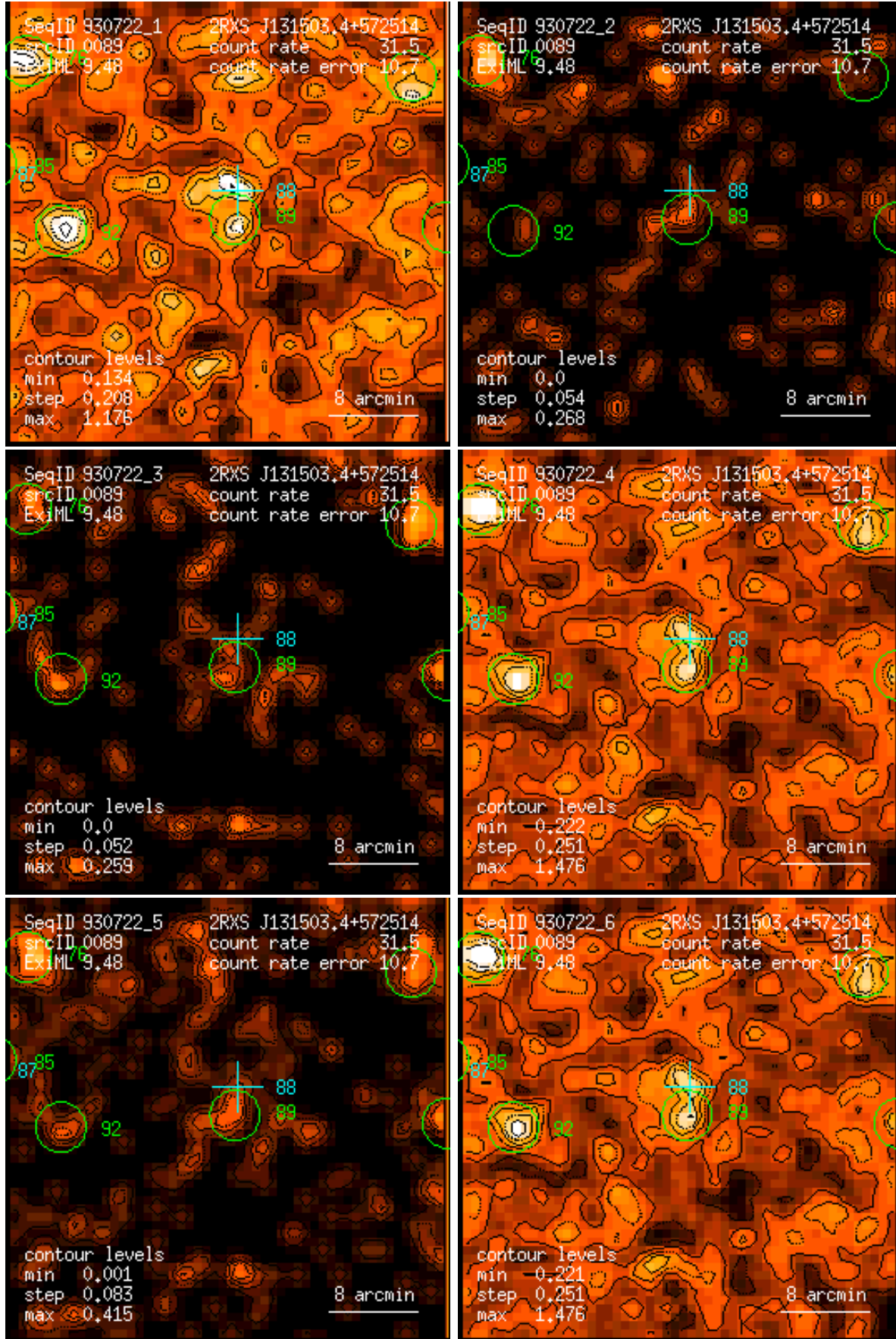
Figure 89: RASS 930722: detection 0089: band rate images, Gaussian filter: (1) PSPC channels 11 – 41, (2) 52 – 90, (3) 91 – 201, (4) 11 – 235, (5) 52 – 201, (6) 11 – 201. Broad band rates in counts/ks. Band rate contour levels in counts/ks/arcmin 2 .
