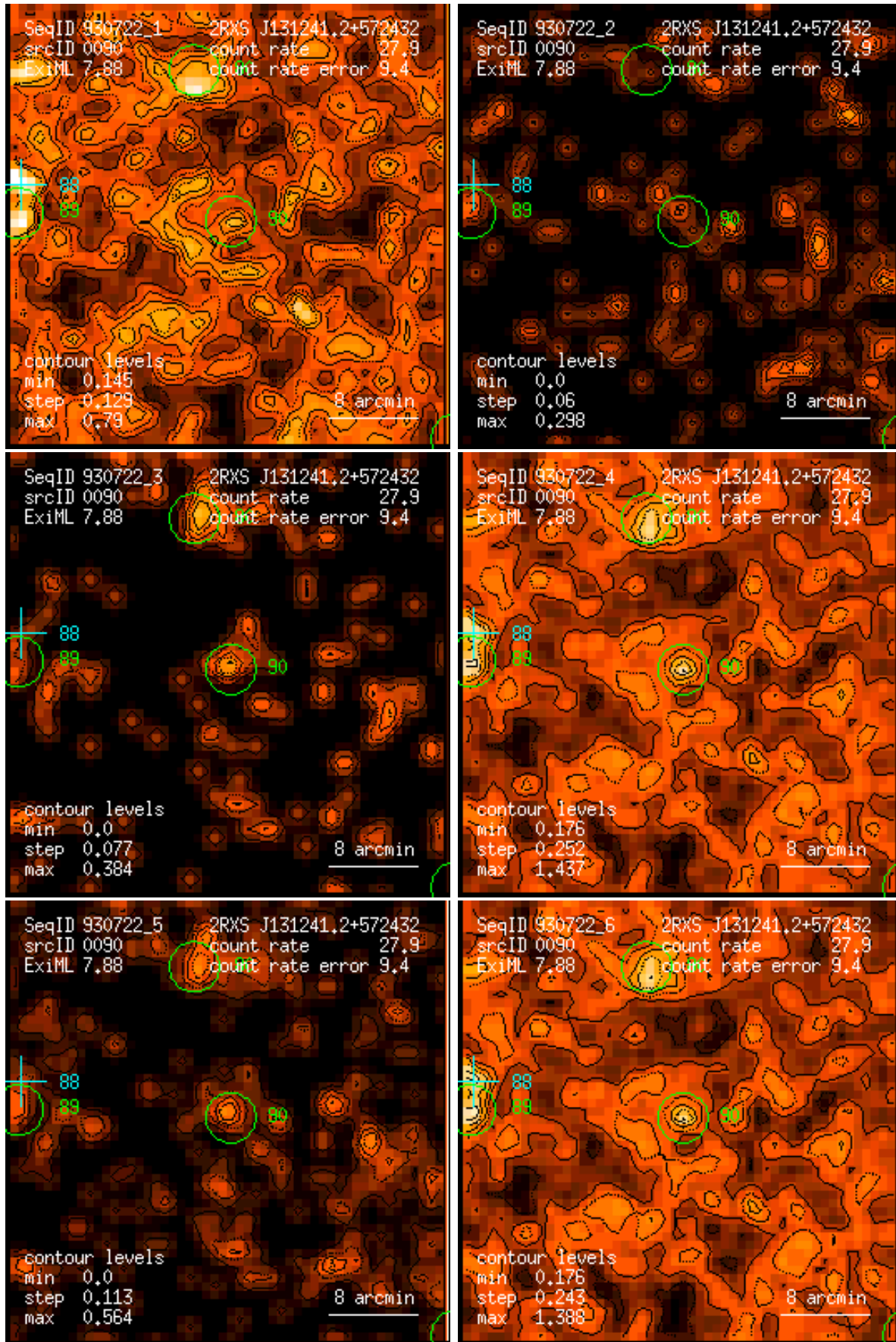
Figure 90: RASS 930722: detection 0090: band rate images, Gaussian filter: (1) PSPC channels 11 – 41, (2) 52 – 90, (3) 91 – 201, (4) 11 – 235, (5) 52 – 201, (6) 11 – 201. Broad band rates in counts/ks. Band rate contour levels in counts/ks/arcmin 2 .
