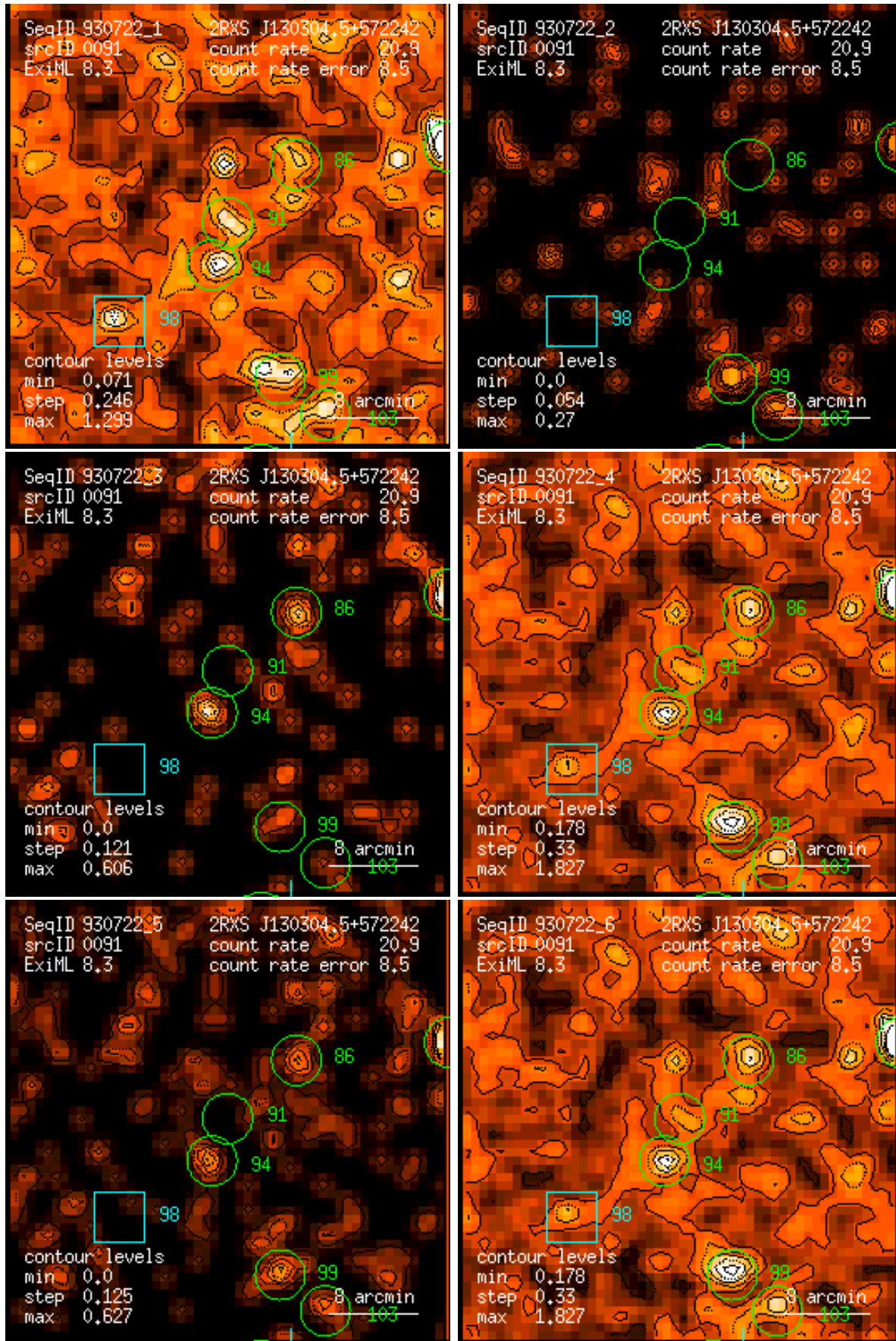
Figure 91: RASS 930722: detection 0091: band rate images, Gaussian filter: (1) PSPC channels 11 – 41, (2) 52 – 90, (3) 91 – 201, (4) 11 – 235, (5) 52 – 201, (6) 11 – 201. Broad band rates in counts/ks. Band rate contour levels in counts/ks/arcmin 2 .
