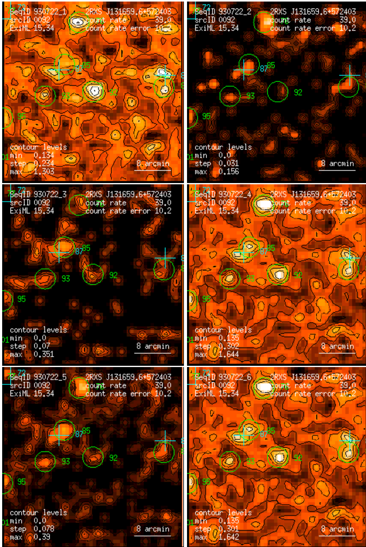
Figure 92: RASS 930722: detection 0092: band rate images, Gaussian filter: (1) PSPC channels 11 – 41, (2) 52 – 90, (3) 91 – 201, (4) 11 – 235, (5) 52 – 201, (6) 11 – 201. Broad band rates in counts/ks. Band rate contour levels in counts/ks/arcmin 2 .
