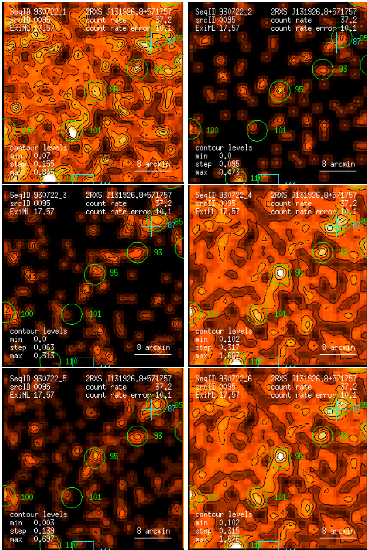
Figure 95: RASS 930722: detection 0095: band rate images, Gaussian filter: (1) PSPC channels 11 – 41, (2) 52 – 90, (3) 91 – 201, (4) 11 – 235, (5) 52 – 201, (6) 11 – 201. Broad band rates in counts/ks. Band rate contour levels in counts/ks/arcmin 2 .
