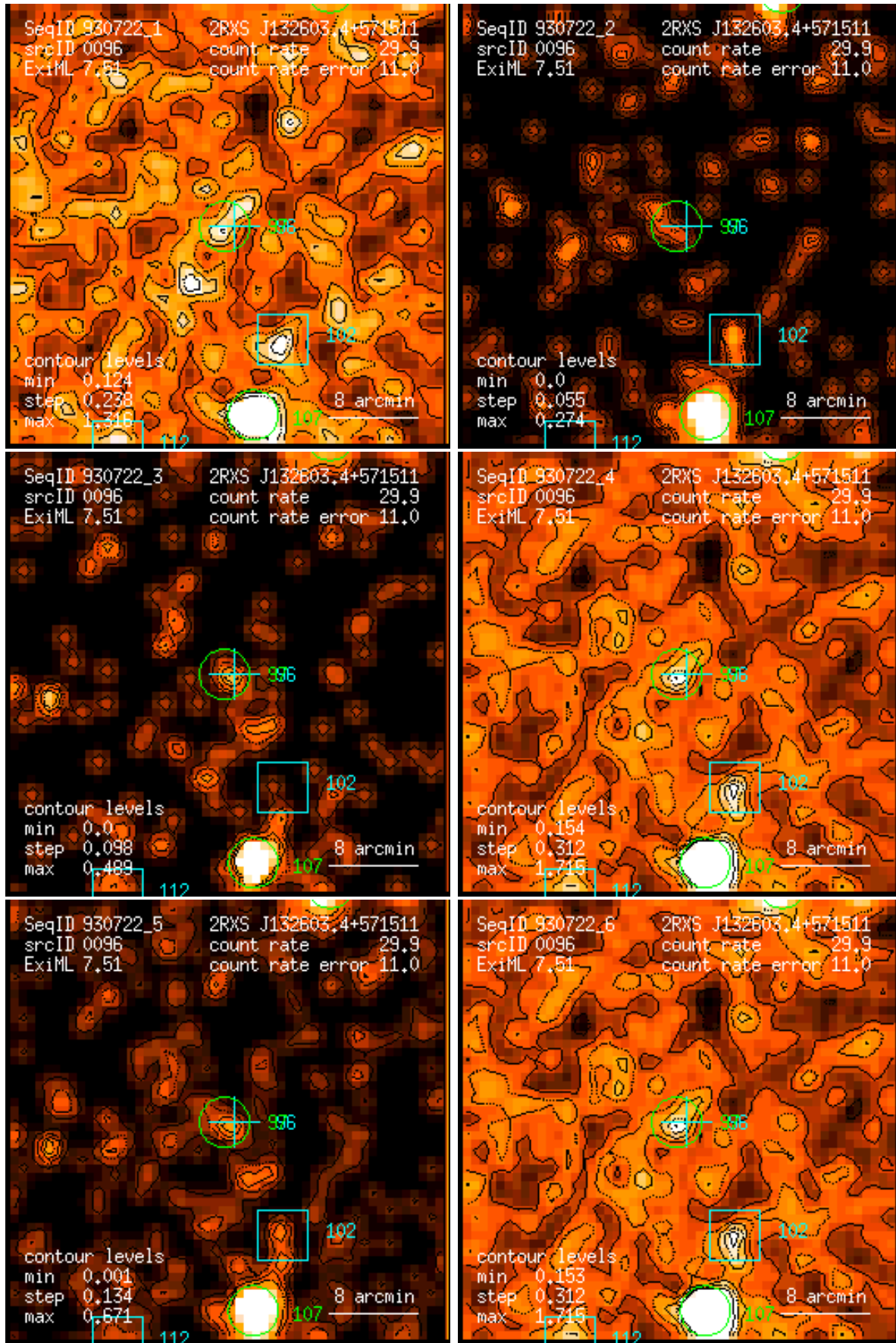
Figure 96: RASS 930722: detection 0096: band rate images, Gaussian filter: (1) PSPC channels 11 – 41, (2) 52 – 90, (3) 91 – 201, (4) 11 – 235, (5) 52 – 201, (6) 11 – 201. Broad band rates in counts/ks. Band rate contour levels in counts/ks/arcmin 2 .
