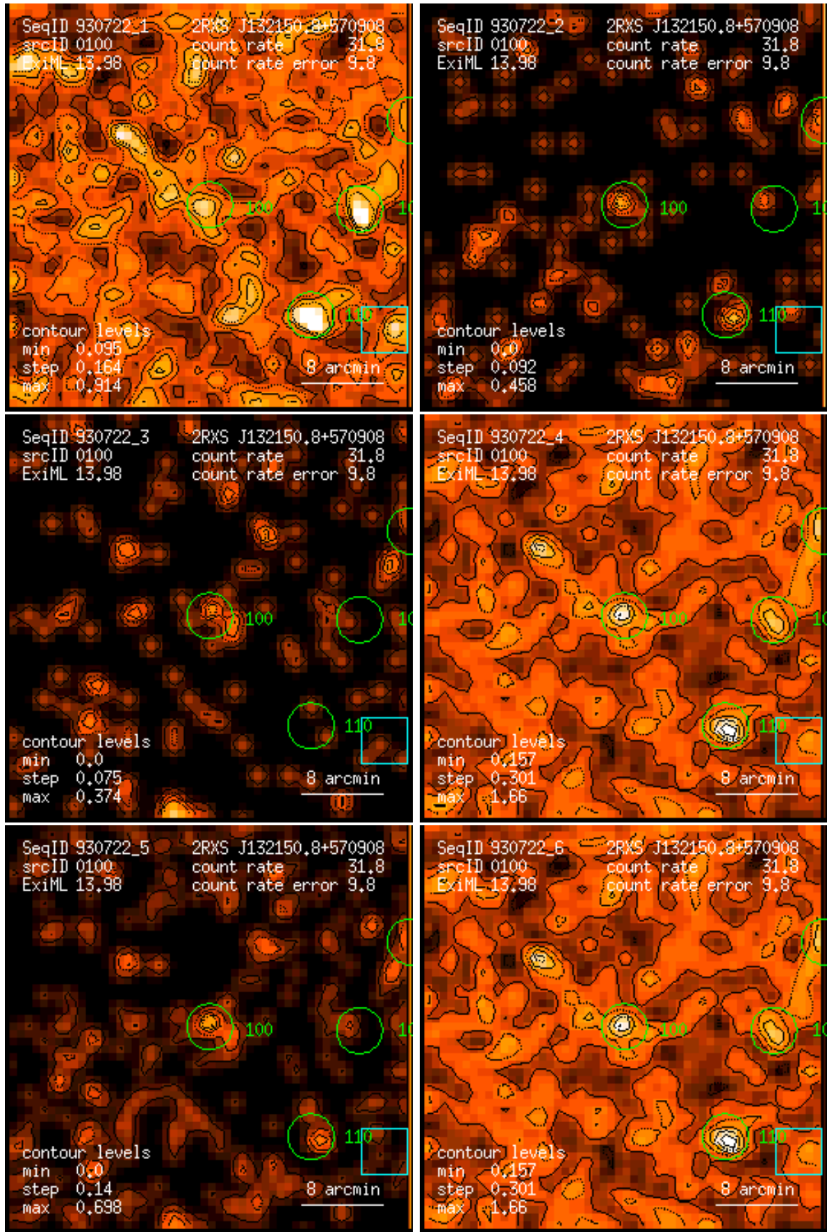
Figure 100: RASS 930722: detection 0100: band rate images, Gaussian filter: (1) PSPC channels 11 – 41, (2) 52 – 90, (3) 91 – 201, (4) 11 – 235, (5) 52 – 201, (6) 11 – 201. Broad band rates in counts/ks. Band rate contour levels in counts/ks/arcmin 2 .
