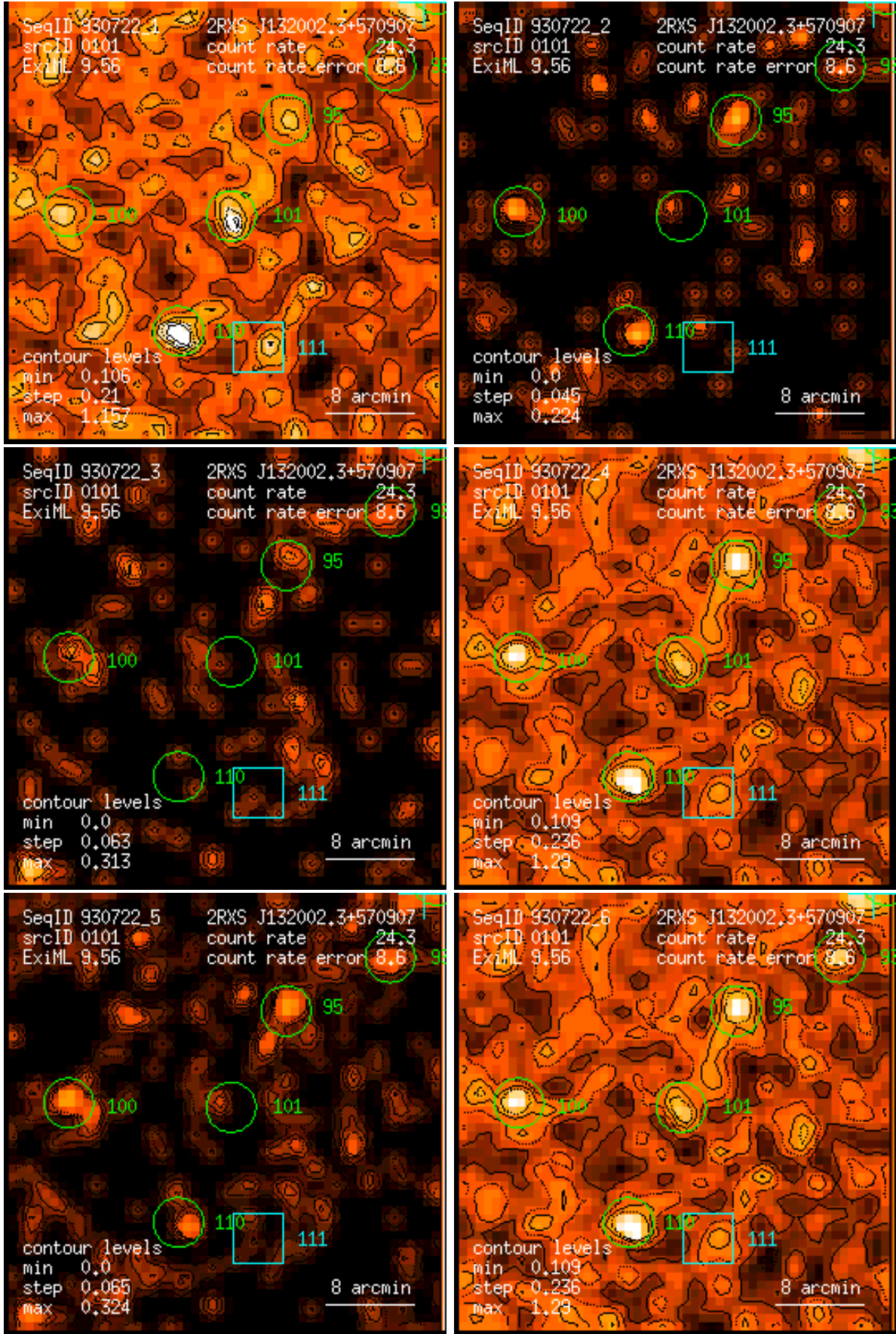
Figure 101: RASS 930722: detection 0101: band rate images, Gaussian filter: (1) PSPC channels 11 – 41, (2) 52 – 90, (3) 91 – 201, (4) 11 – 235, (5) 52 – 201, (6) 11 – 201. Broad band rates in counts/ks. Band rate contour levels in counts/ks/arcmin 2 .
