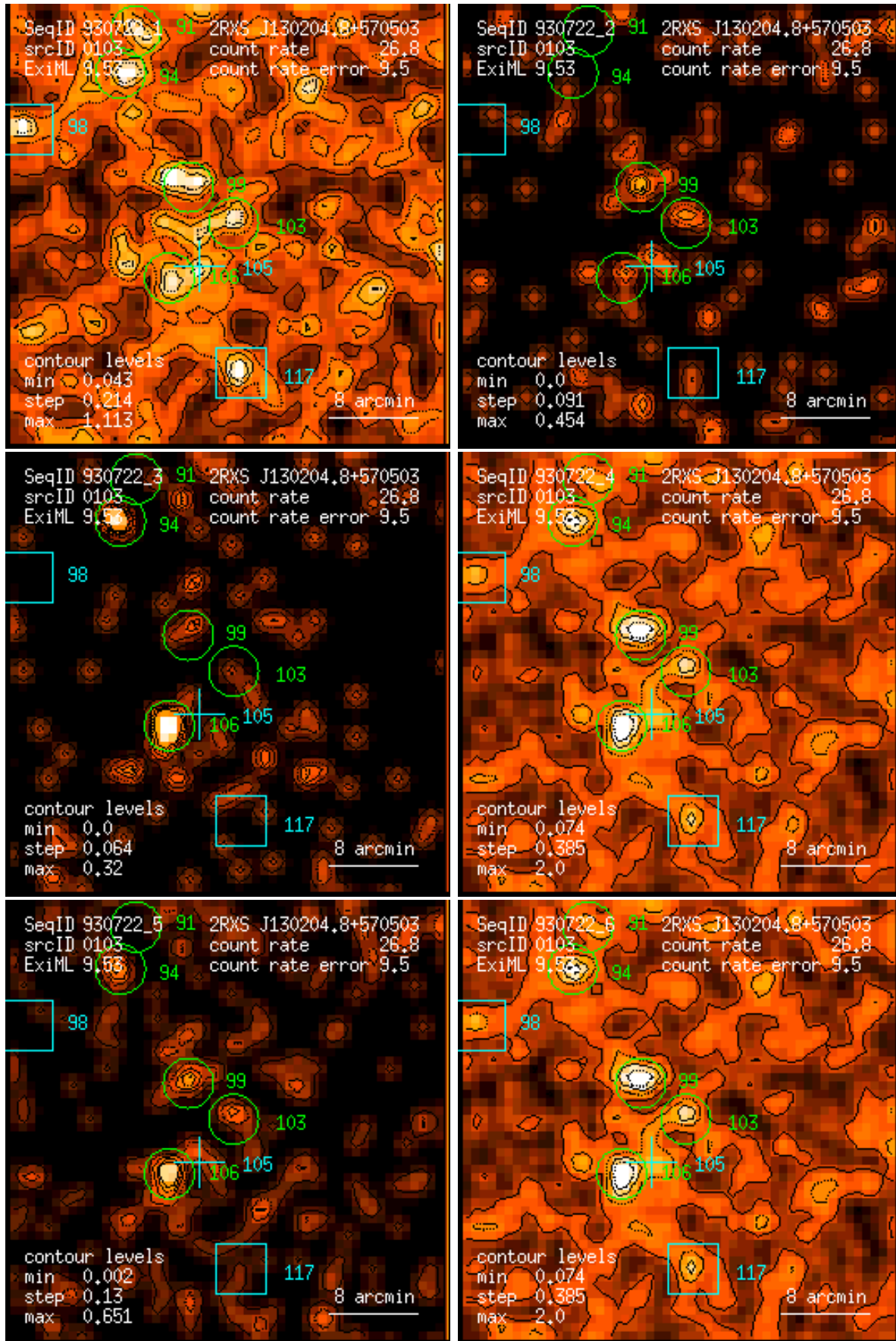
Figure 103: RASS 930722: detection 0103: band rate images, Gaussian filter: (1) PSPC channels 11 – 41, (2) 52 – 90, (3) 91 – 201, (4) 11 – 235, (5) 52 – 201, (6) 11 – 201. Broad band rates in counts/ks. Band rate contour levels in counts/ks/arcmin 2 .
