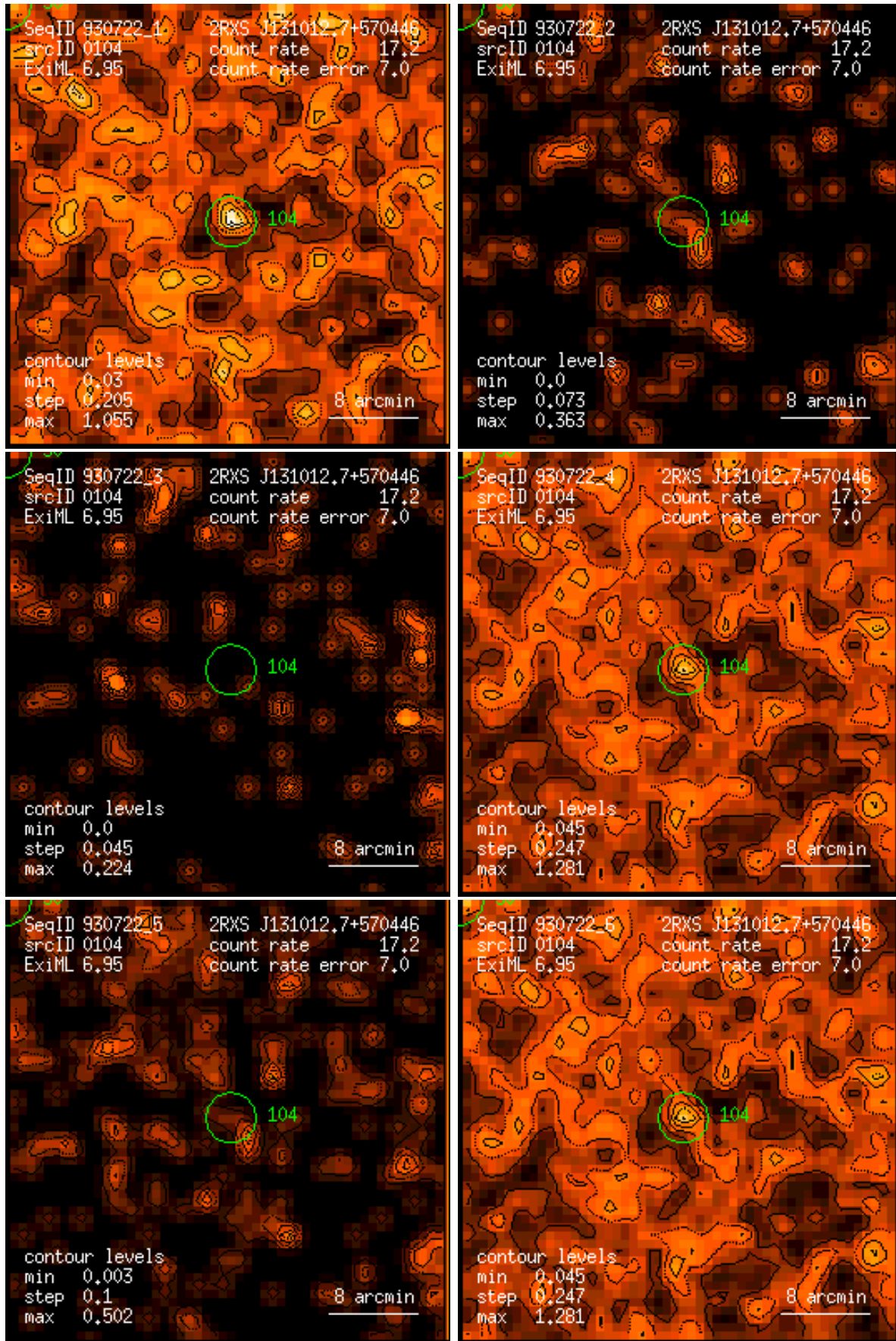
Figure 104: RASS 930722: detection 0104: band rate images, Gaussian filter: (1) PSPC channels 11 – 41, (2) 52 – 90, (3) 91 – 201, (4) 11 – 235, (5) 52 – 201, (6) 11 – 201. Broad band rates in counts/ks. Band rate contour levels in counts/ks/arcmin 2 .
