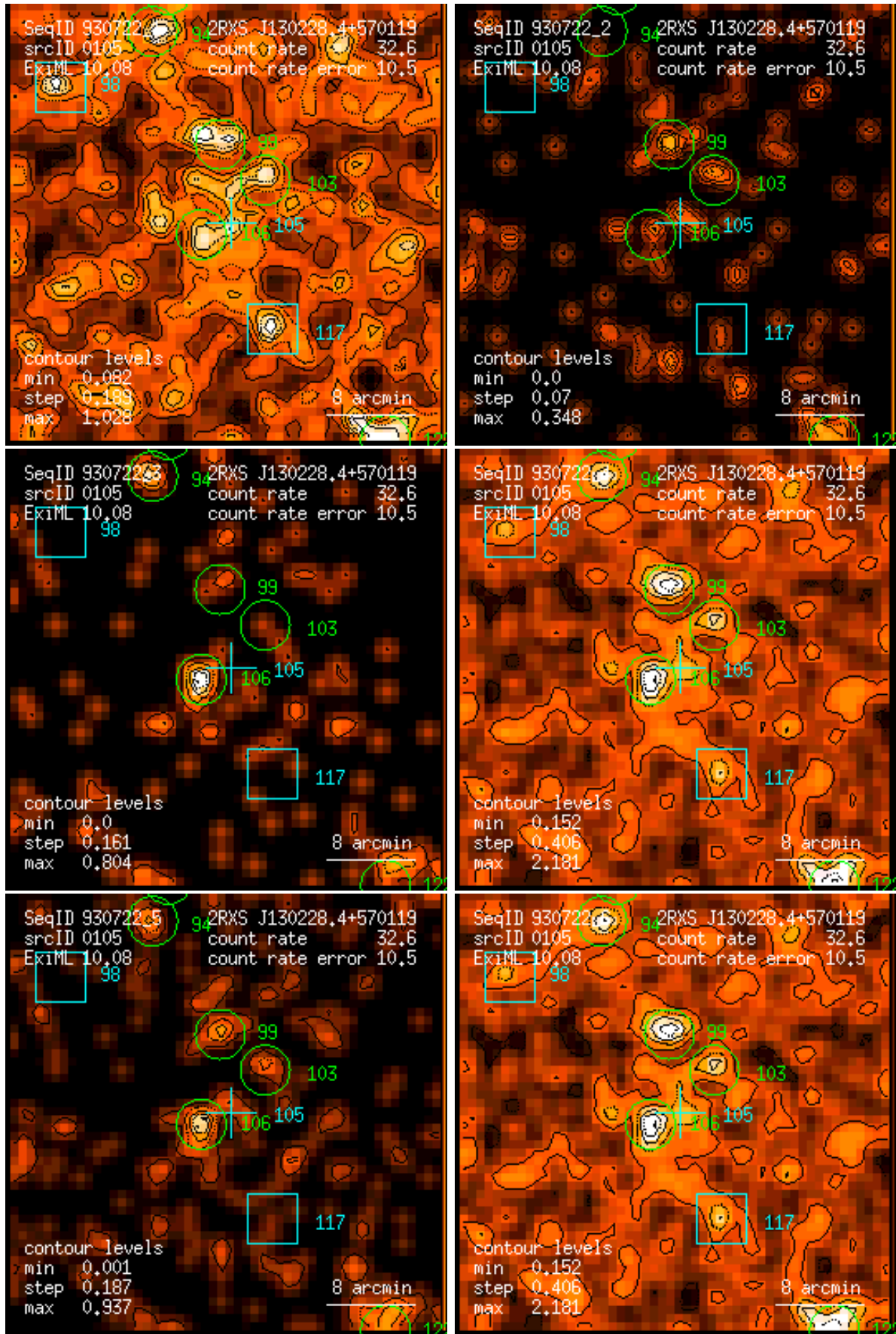
Figure 105: RASS 930722: detection 0105: band rate images, Gaussian filter: (1) PSPC channels 11 – 41, (2) 52 – 90, (3) 91 – 201, (4) 11 – 235, (5) 52 – 201, (6) 11 – 201. Broad band rates in counts/ks. Band rate contour levels in counts/ks/arcmin 2 .
