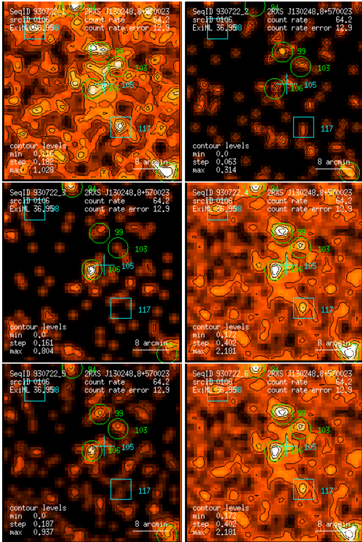
Figure 106: RASS 930722: detection 0106: band rate images, Gaussian filter: (1) PSPC channels 11 – 41, (2) 52 – 90, (3) 91 – 201, (4) 11 – 235, (5) 52 – 201, (6) 11 – 201. Broad band rates in counts/ks. Band rate contour levels in counts/ks/arcmin 2 .
