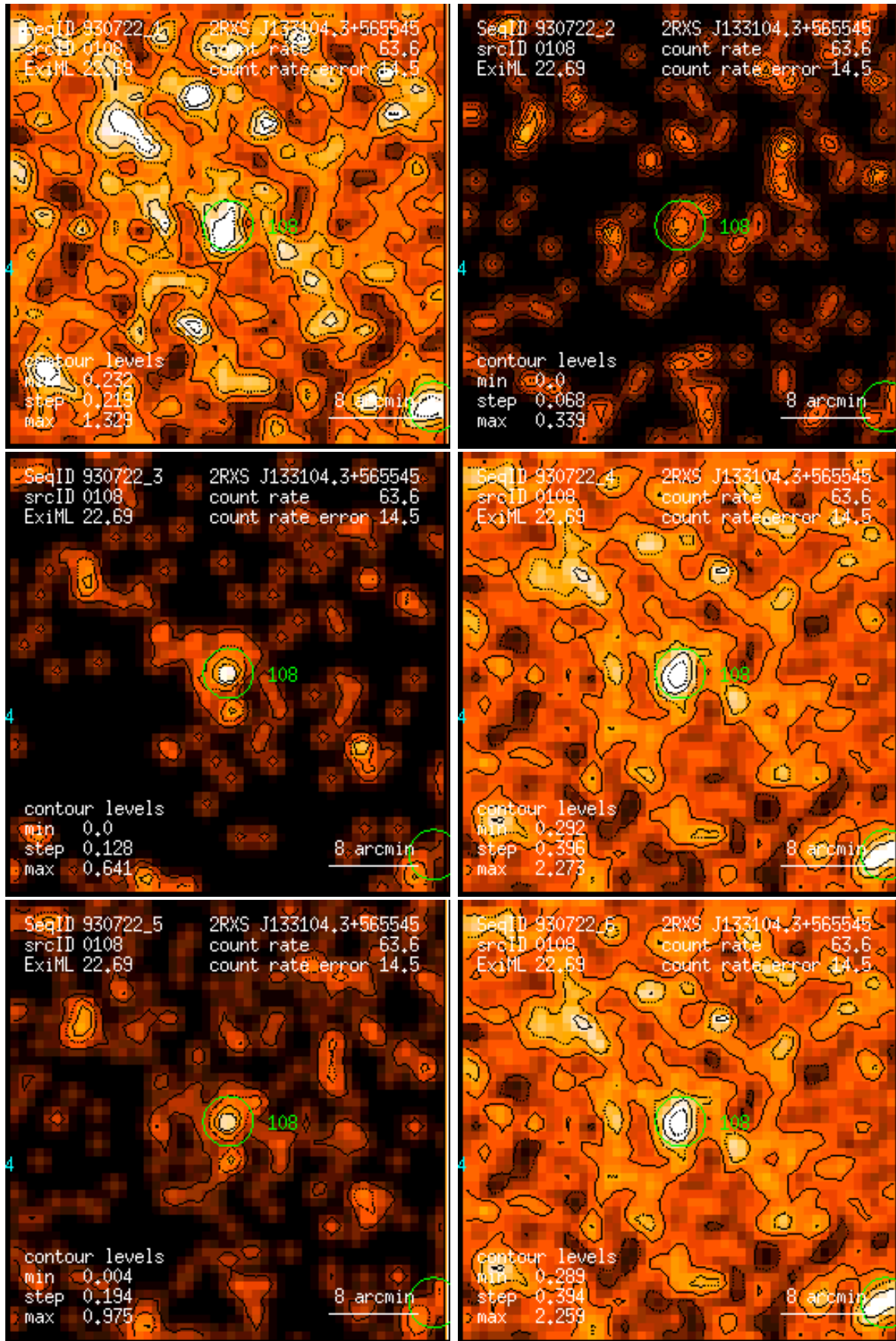
Figure 108: RASS 930722: detection 0108: band rate images, Gaussian filter: (1) PSPC channels 11 – 41, (2) 52 – 90, (3) 91 – 201, (4) 11 – 235, (5) 52 – 201, (6) 11 – 201. Broad band rates in counts/ks. Band rate contour levels in counts/ks/arcmin 2 .
