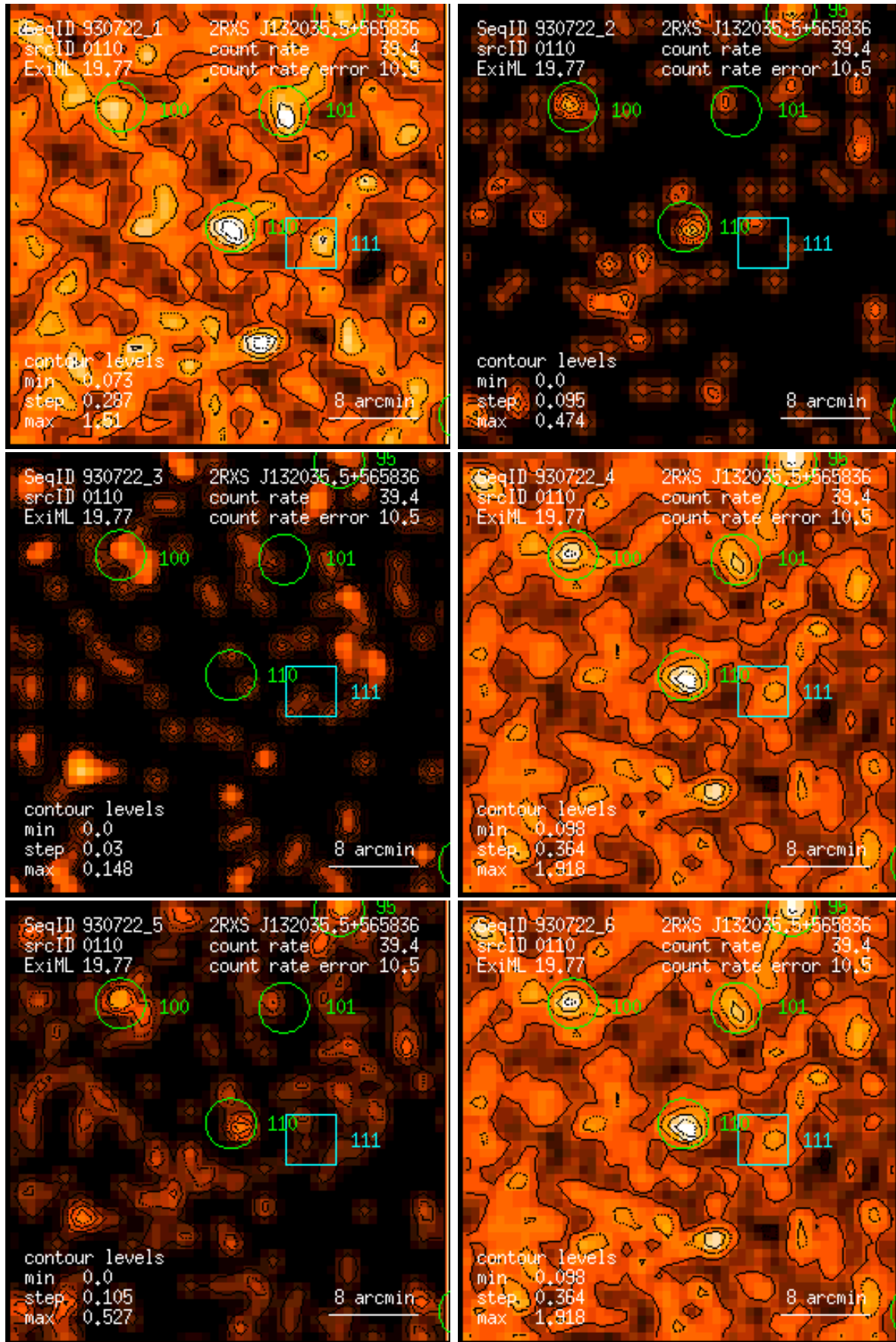
Figure 110: RASS 930722: detection 0110: band rate images, Gaussian filter: (1) PSPC channels 11 – 41, (2) 52 – 90, (3) 91 – 201, (4) 11 – 235, (5) 52 – 201, (6) 11 – 201. Broad band rates in counts/ks. Band rate contour levels in counts/ks/arcmin 2 .
