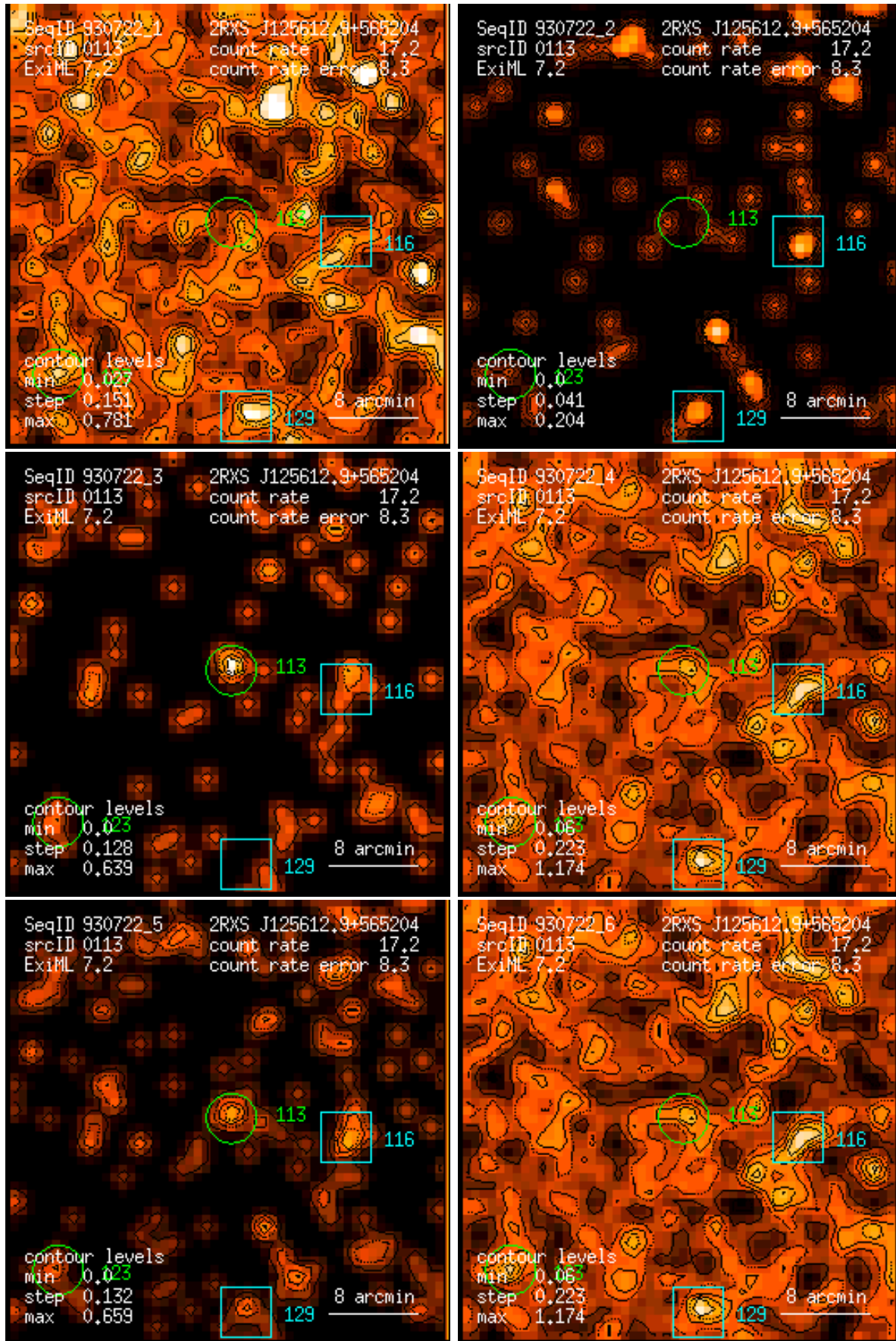
Figure 113: RASS 930722: detection 0113: band rate images, Gaussian filter: (1) PSPC channels 11 – 41, (2) 52 – 90, (3) 91 – 201, (4) 11 – 235, (5) 52 – 201, (6) 11 – 201. Broad band rates in counts/ks. Band rate contour levels in counts/ks/arcmin 2 .
