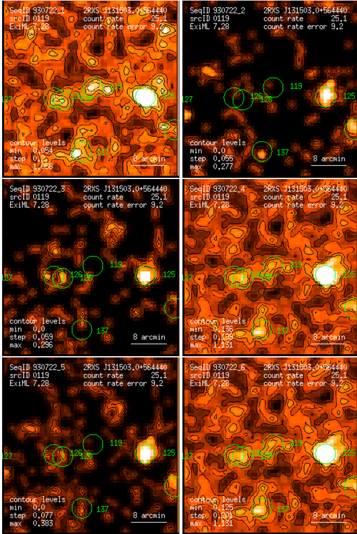
Figure 119: RASS 930722: detection 0119: band rate images, Gaussian filter: (1) PSPC channels 11 – 41, (2) 52 – 90, (3) 91 – 201, (4) 11 – 235, (5) 52 – 201, (6) 11 – 201. Broad band rates in counts/ks. Band rate contour levels in counts/ks/arcmin 2 .
