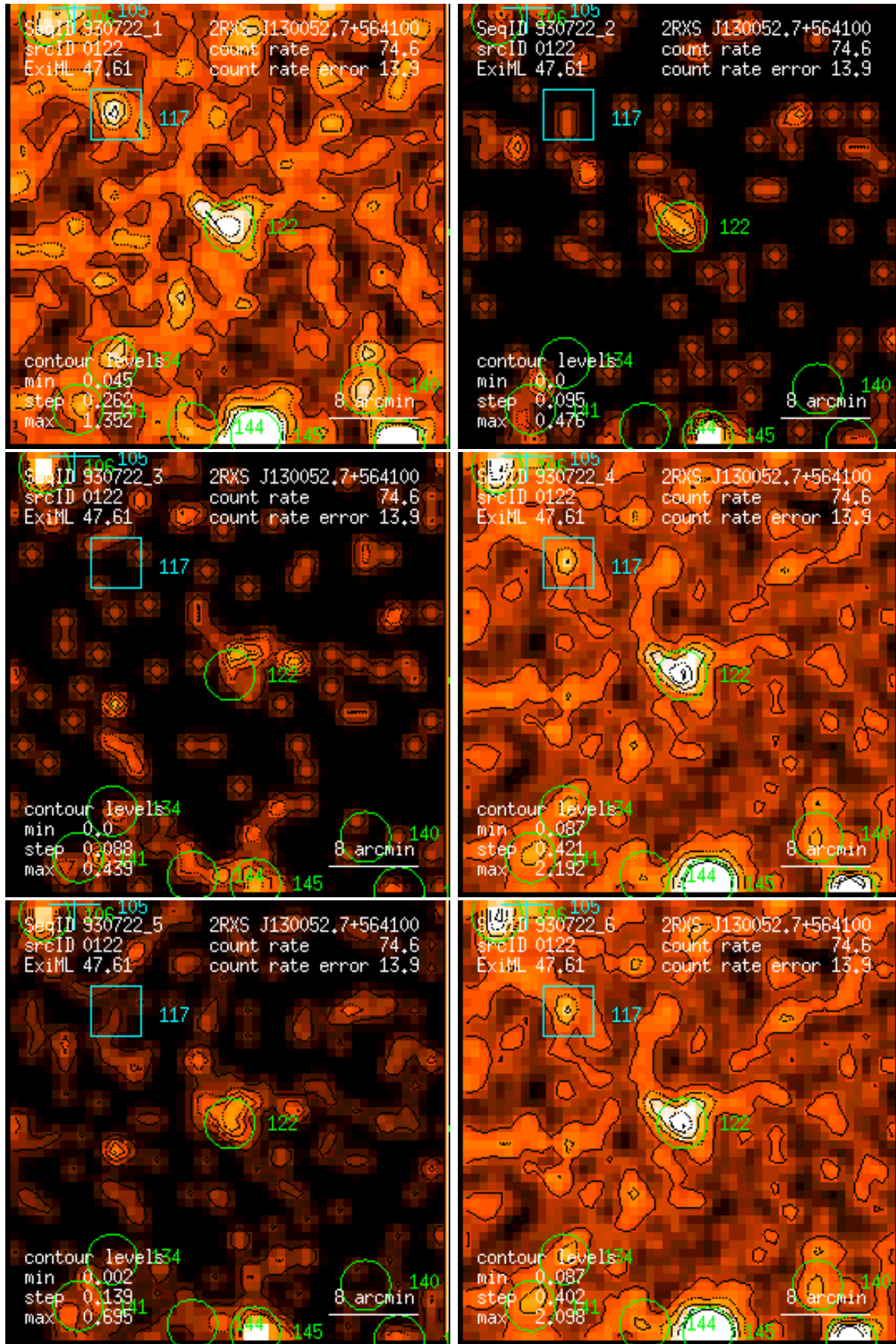
Figure 122: RASS 930722: detection 0122: band rate images, Gaussian filter: (1) PSPC channels 11 – 41, (2) 52 – 90, (3) 91 – 201, (4) 11 – 235, (5) 52 – 201, (6) 11 – 201. Broad band rates in counts/ks. Band rate contour levels in counts/ks/arcmin 2 .
