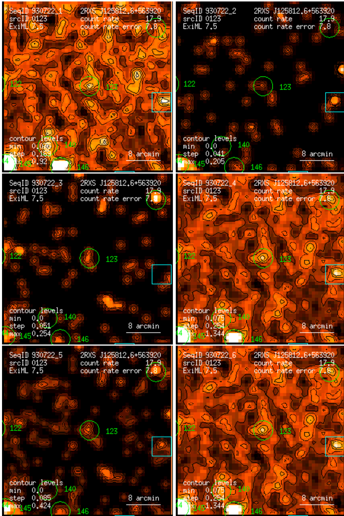
Figure 123: RASS 930722: detection 0123: band rate images, Gaussian filter: (1) PSPC channels 11 – 41, (2) 52 – 90, (3) 91 – 201, (4) 11 – 235, (5) 52 – 201, (6) 11 – 201. Broad band rates in counts/ks. Band rate contour levels in counts/ks/arcmin 2 .
