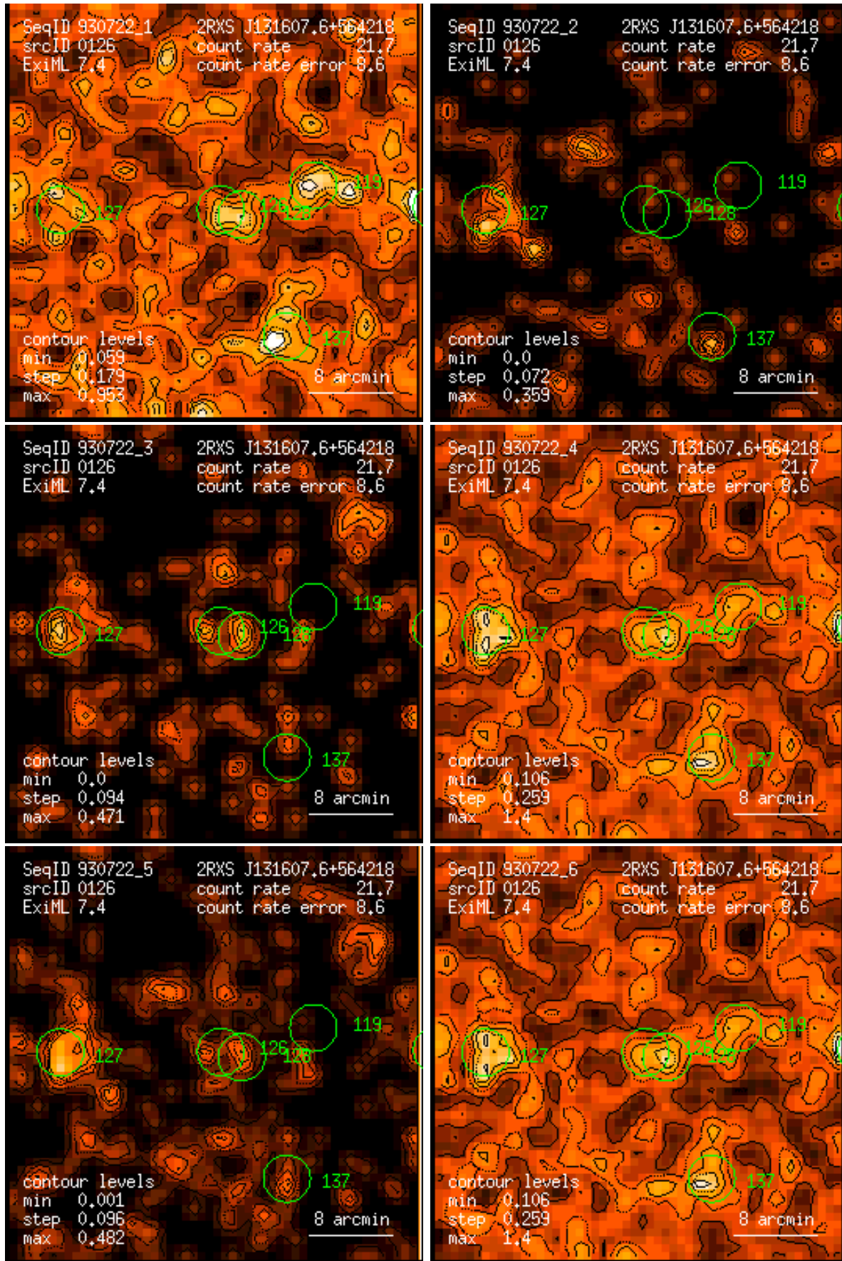
Figure 126: RASS 930722: detection 0126: band rate images, Gaussian filter: (1) PSPC channels 11 – 41, (2) 52 – 90, (3) 91 – 201, (4) 11 – 235, (5) 52 – 201, (6) 11 – 201. Broad band rates in counts/ks. Band rate contour levels in counts/ks/arcmin 2 .
