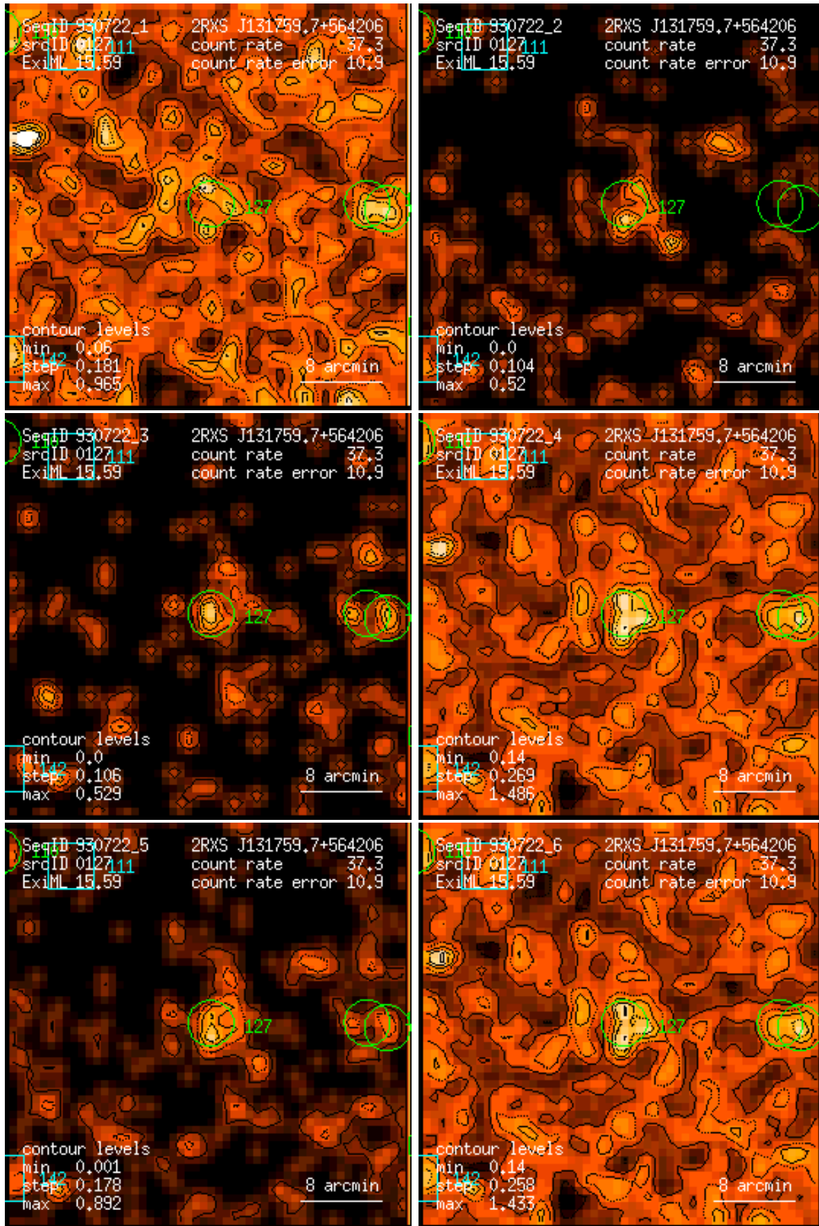
Figure 127: RASS 930722: detection 0127: band rate images, Gaussian filter: (1) PSPC channels 11 – 41, (2) 52 – 90, (3) 91 – 201, (4) 11 – 235, (5) 52 – 201, (6) 11 – 201. Broad band rates in counts/ks. Band rate contour levels in counts/ks/arcmin 2 .
