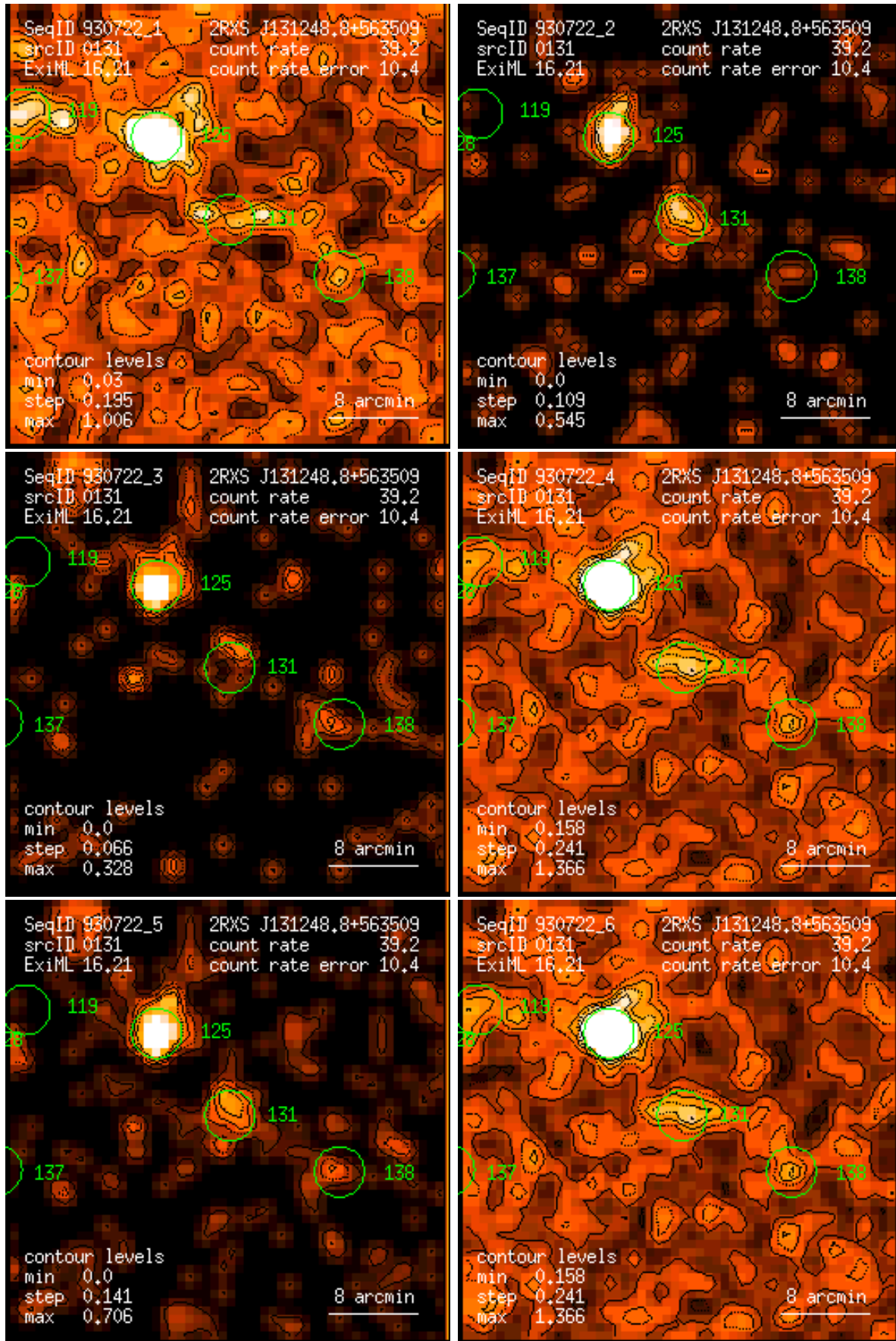
Figure 131: RASS 930722: detection 0131: band rate images, Gaussian filter: (1) PSPC channels 11 – 41, (2) 52 – 90, (3) 91 – 201, (4) 11 – 235, (5) 52 – 201, (6) 11 – 201. Broad band rates in counts/ks. Band rate contour levels in counts/ks/arcmin 2 .
