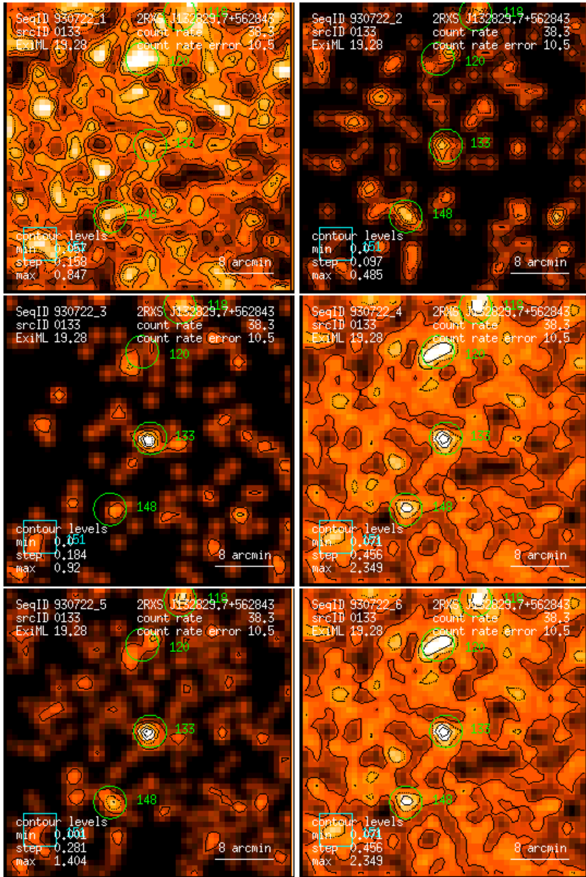
Figure 133: RASS 930722: detection 0133: band rate images, Gaussian filter: (1) PSPC channels 11 – 41, (2) 52 – 90, (3) 91 – 201, (4) 11 – 235, (5) 52 – 201, (6) 11 – 201. Broad band rates in counts/ks. Band rate contour levels in counts/ks/arcmin 2 .
