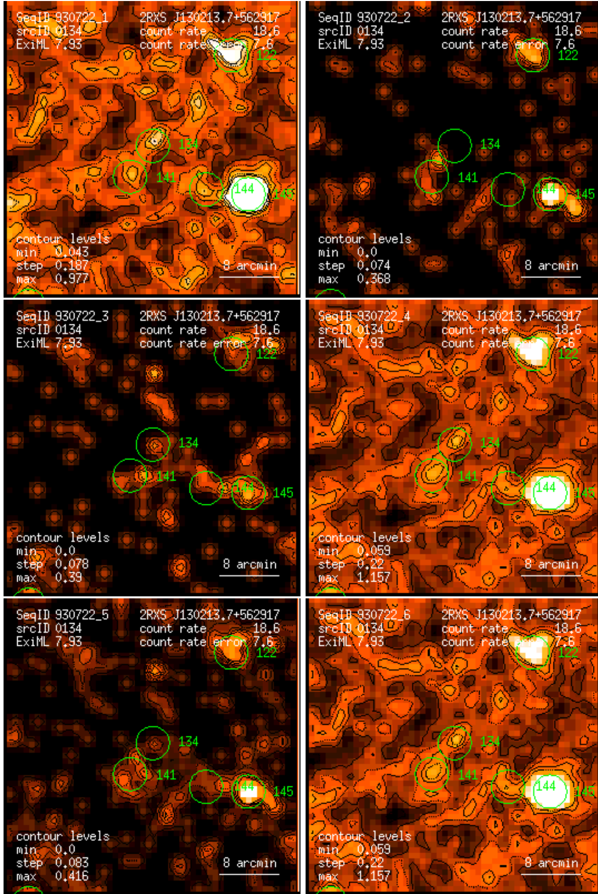
Figure 134: RASS 930722: detection 0134: band rate images, Gaussian filter: (1) PSPC channels 11 – 41, (2) 52 – 90, (3) 91 – 201, (4) 11 – 235, (5) 52 – 201, (6) 11 – 201. Broad band rates in counts/ks. Band rate contour levels in counts/ks/arcmin 2 .
