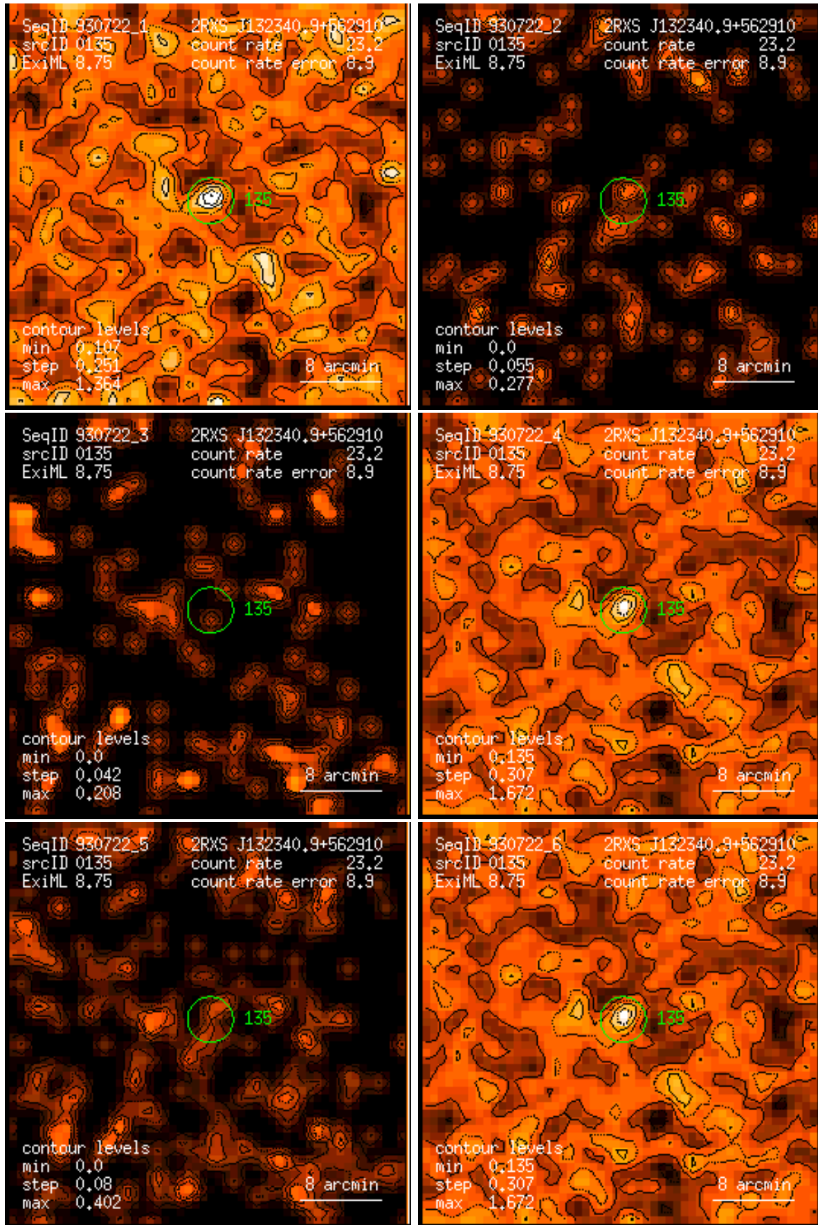
Figure 135: RASS 930722: detection 0135: band rate images, Gaussian filter: (1) PSPC channels 11 – 41, (2) 52 – 90, (3) 91 – 201, (4) 11 – 235, (5) 52 – 201, (6) 11 – 201. Broad band rates in counts/ks. Band rate contour levels in counts/ks/arcmin 2 .
