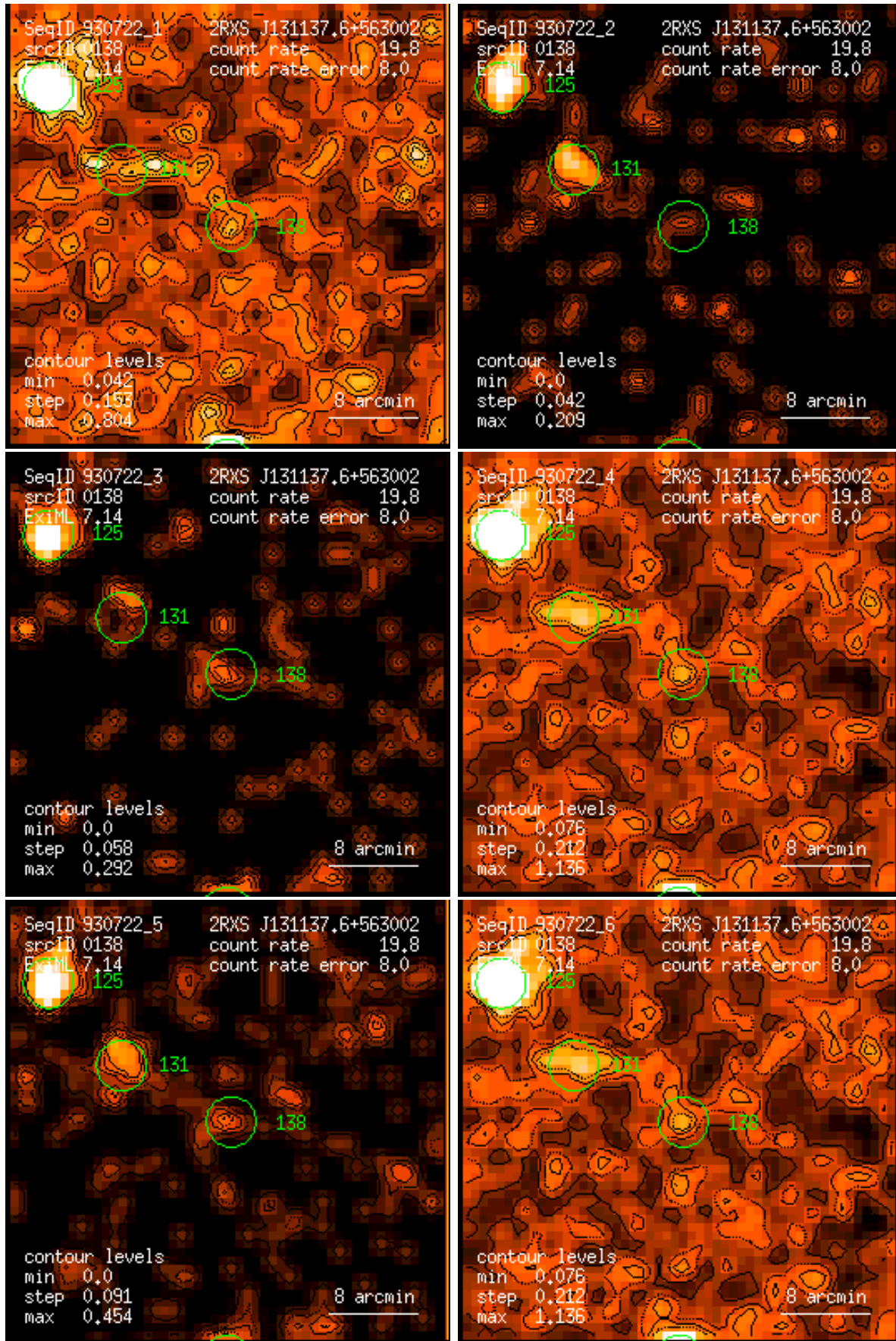
Figure 138: RASS 930722: detection 0138: band rate images, Gaussian filter: (1) PSPC channels 11 – 41, (2) 52 – 90, (3) 91 – 201, (4) 11 – 235, (5) 52 – 201, (6) 11 – 201. Broad band rates in counts/ks. Band rate contour levels in counts/ks/arcmin 2 .
