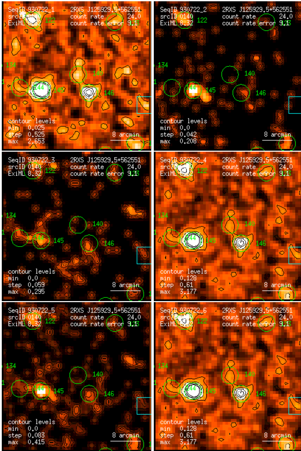
Figure 140: RASS 930722: detection 0140: band rate images, Gaussian filter: (1) PSPC channels 11 – 41, (2) 52 – 90, (3) 91 – 201, (4) 11 – 235, (5) 52 – 201, (6) 11 – 201. Broad band rates in counts/ks. Band rate contour levels in counts/ks/arcmin 2 .
