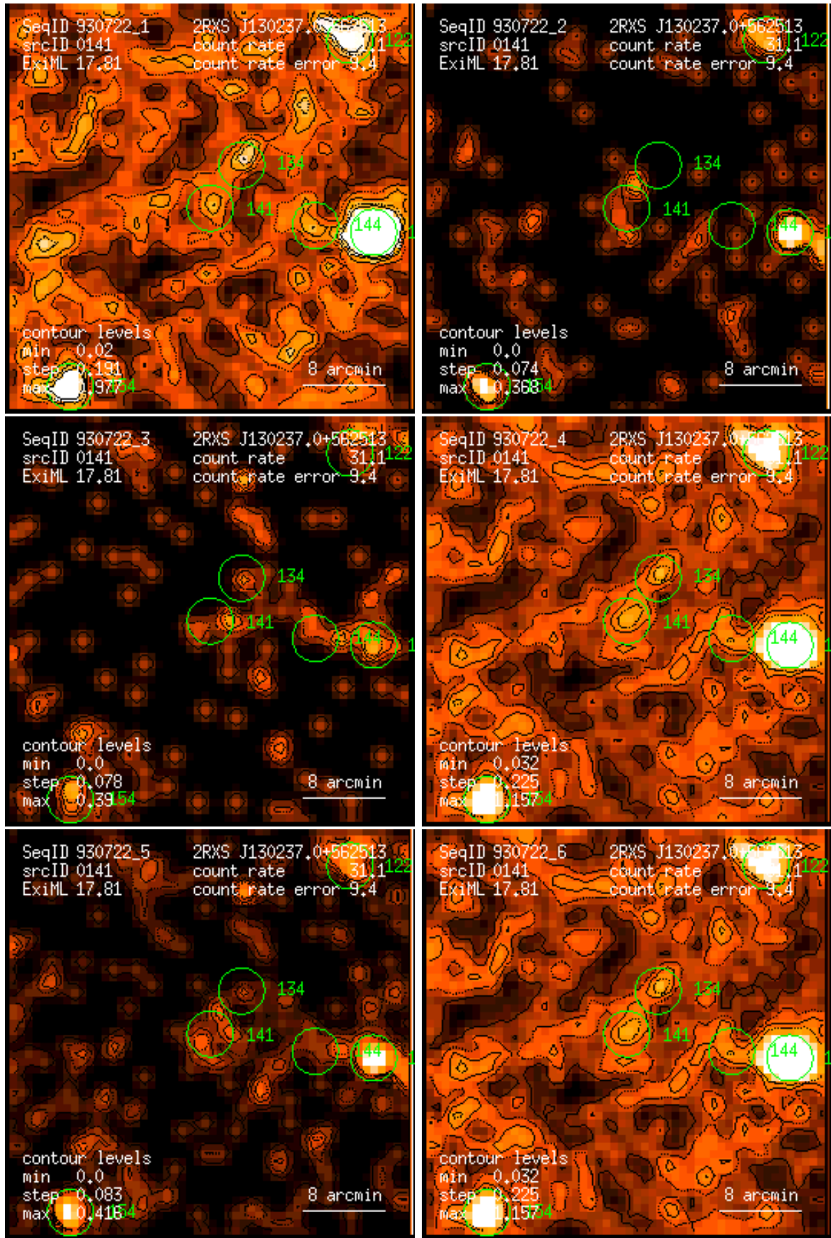
Figure 141: RASS 930722: detection 0141: band rate images, Gaussian filter: (1) PSPC channels 11 – 41, (2) 52 – 90, (3) 91 – 201, (4) 11 – 235, (5) 52 – 201, (6) 11 – 201. Broad band rates in counts/ks. Band rate contour levels in counts/ks/arcmin 2 .
