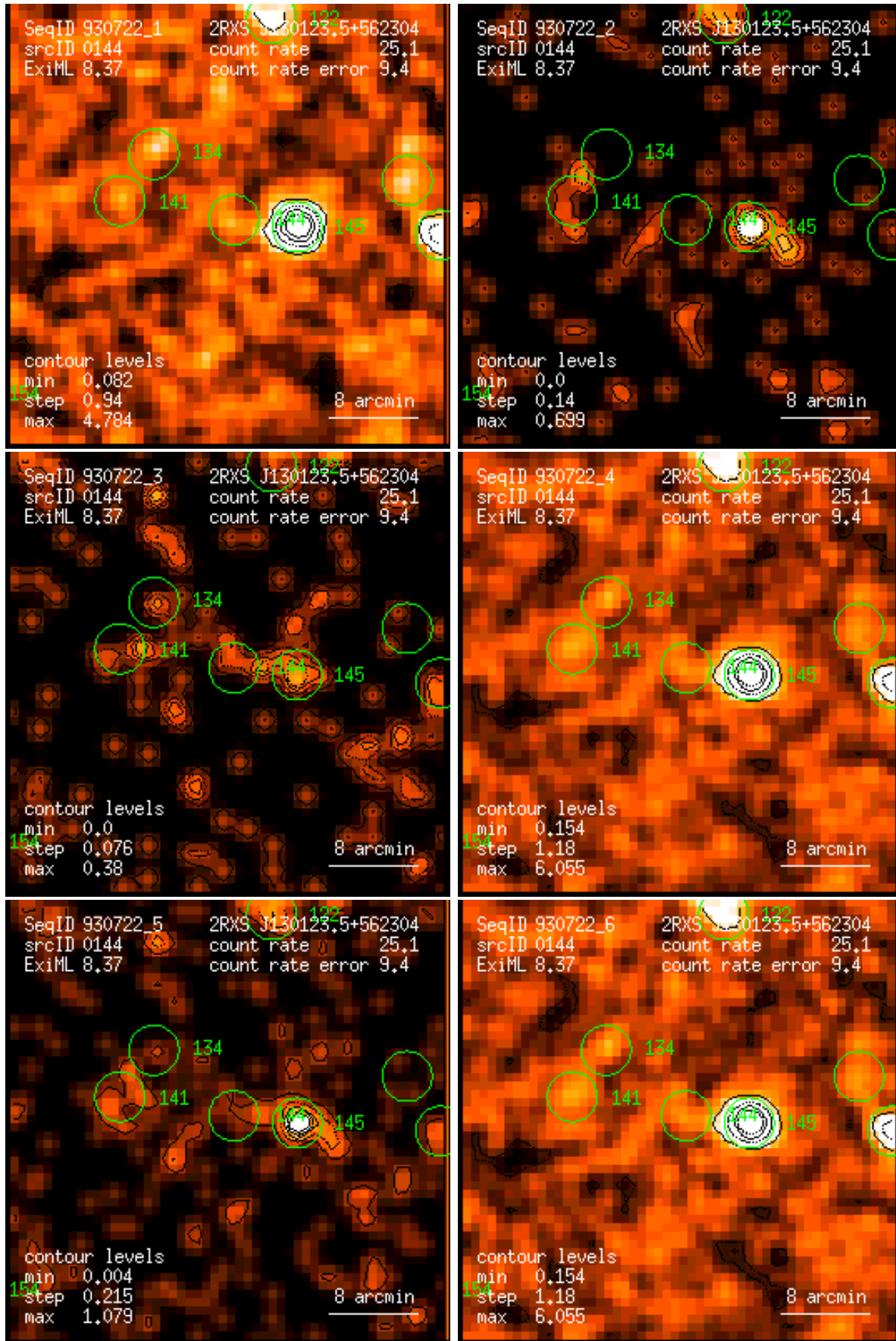
Figure 144: RASS 930722: detection 0144: band rate images, Gaussian filter: (1) PSPC channels 11 – 41, (2) 52 – 90, (3) 91 – 201, (4) 11 – 235, (5) 52 – 201, (6) 11 – 201. Broad band rates in counts/ks. Band rate contour levels in counts/ks/arcmin 2 .
