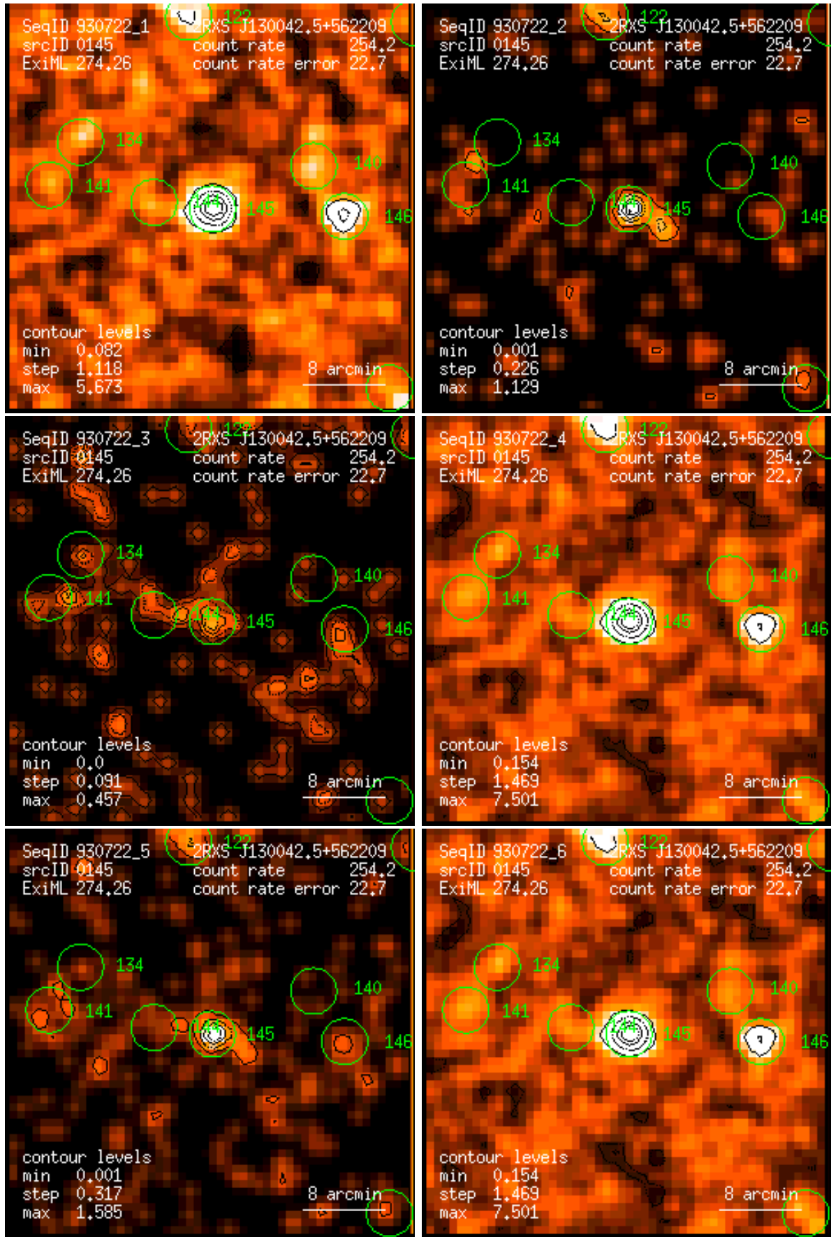
Figure 145: RASS 930722: detection 0145: band rate images, Gaussian filter: (1) PSPC channels 11 – 41, (2) 52 – 90, (3) 91 – 201, (4) 11 – 235, (5) 52 – 201, (6) 11 – 201. Broad band rates in counts/ks. Band rate contour levels in counts/ks/arcmin 2 .
