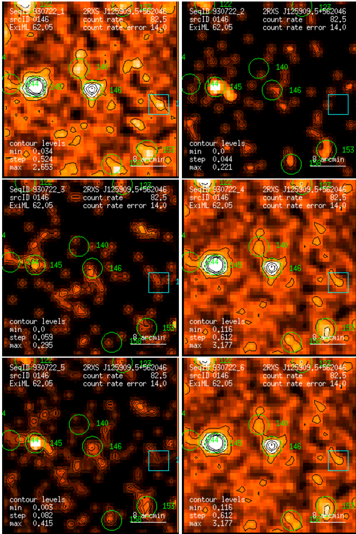
Figure 146: RASS 930722: detection 0146: band rate images, Gaussian filter: (1) PSPC channels 11 – 41, (2) 52 – 90, (3) 91 – 201, (4) 11 – 235, (5) 52 – 201, (6) 11 – 201. Broad band rates in counts/ks. Band rate contour levels in counts/ks/arcmin 2 .
