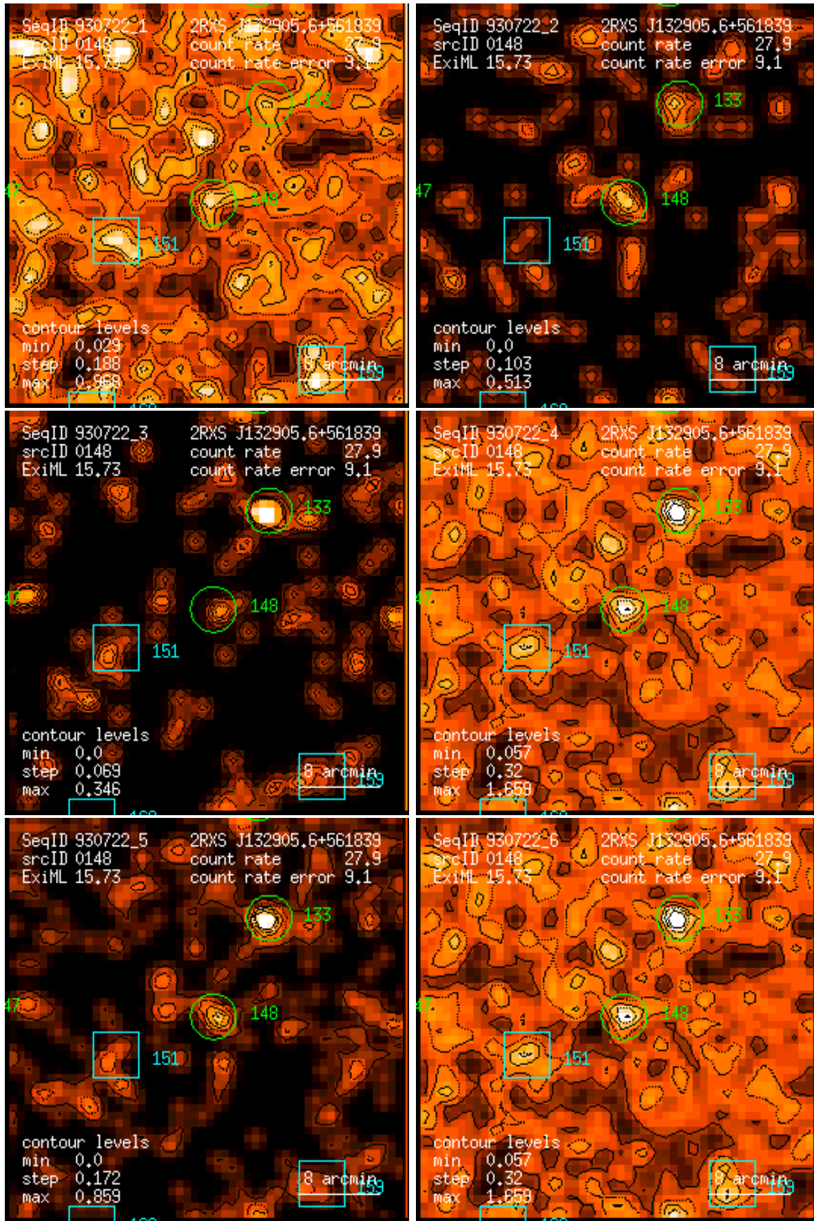
Figure 148: RASS 930722: detection 0148: band rate images, Gaussian filter: (1) PSPC channels 11 – 41, (2) 52 – 90, (3) 91 – 201, (4) 11 – 235, (5) 52 – 201, (6) 11 – 201. Broad band rates in counts/ks. Band rate contour levels in counts/ks/arcmin 2 .
