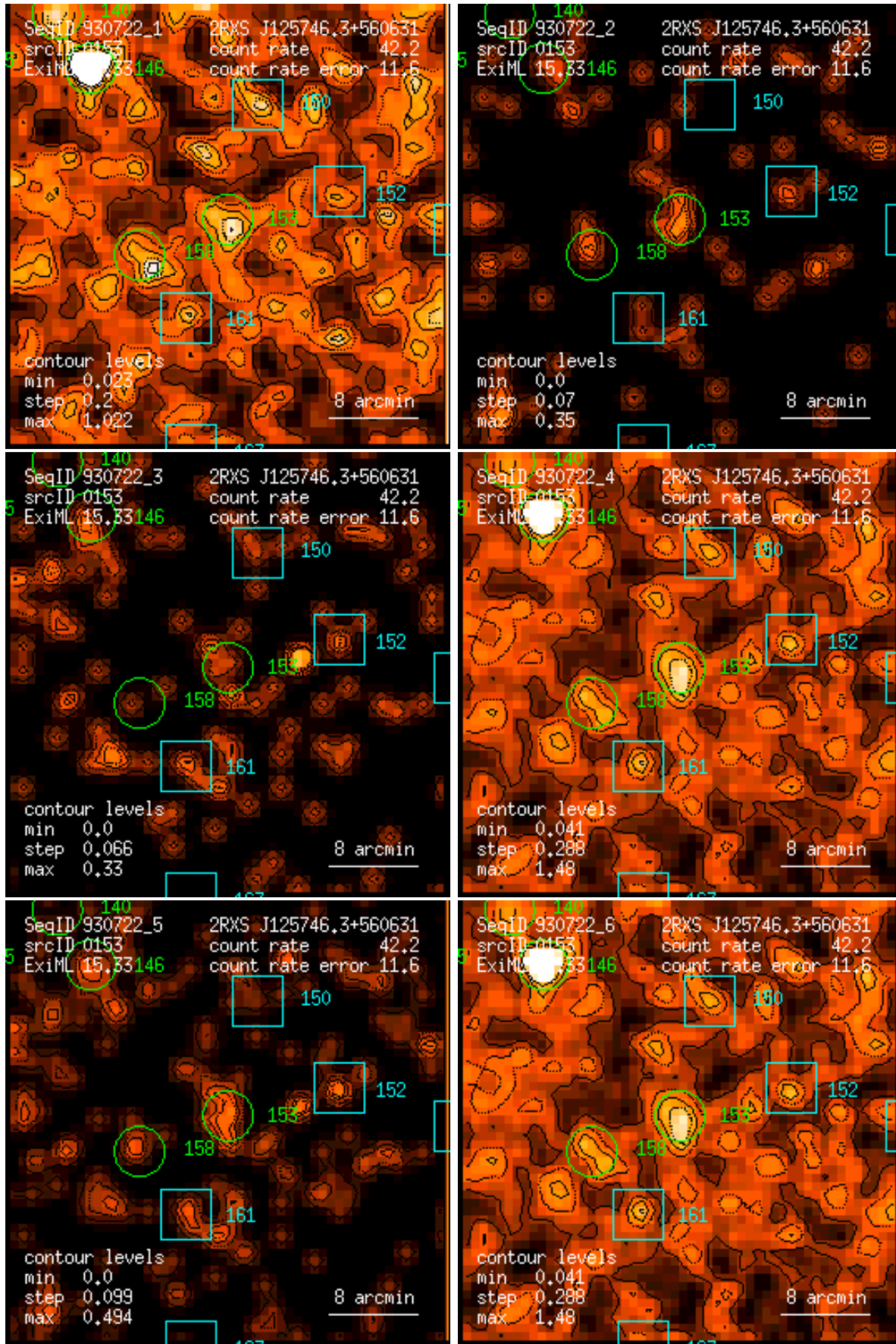
Figure 153: RASS 930722: detection 0153: band rate images, Gaussian filter: (1) PSPC channels 11 – 41, (2) 52 – 90, (3) 91 – 201, (4) 11 – 235, (5) 52 – 201, (6) 11 – 201. Broad band rates in counts/ks. Band rate contour levels in counts/ks/arcmin 2 .
