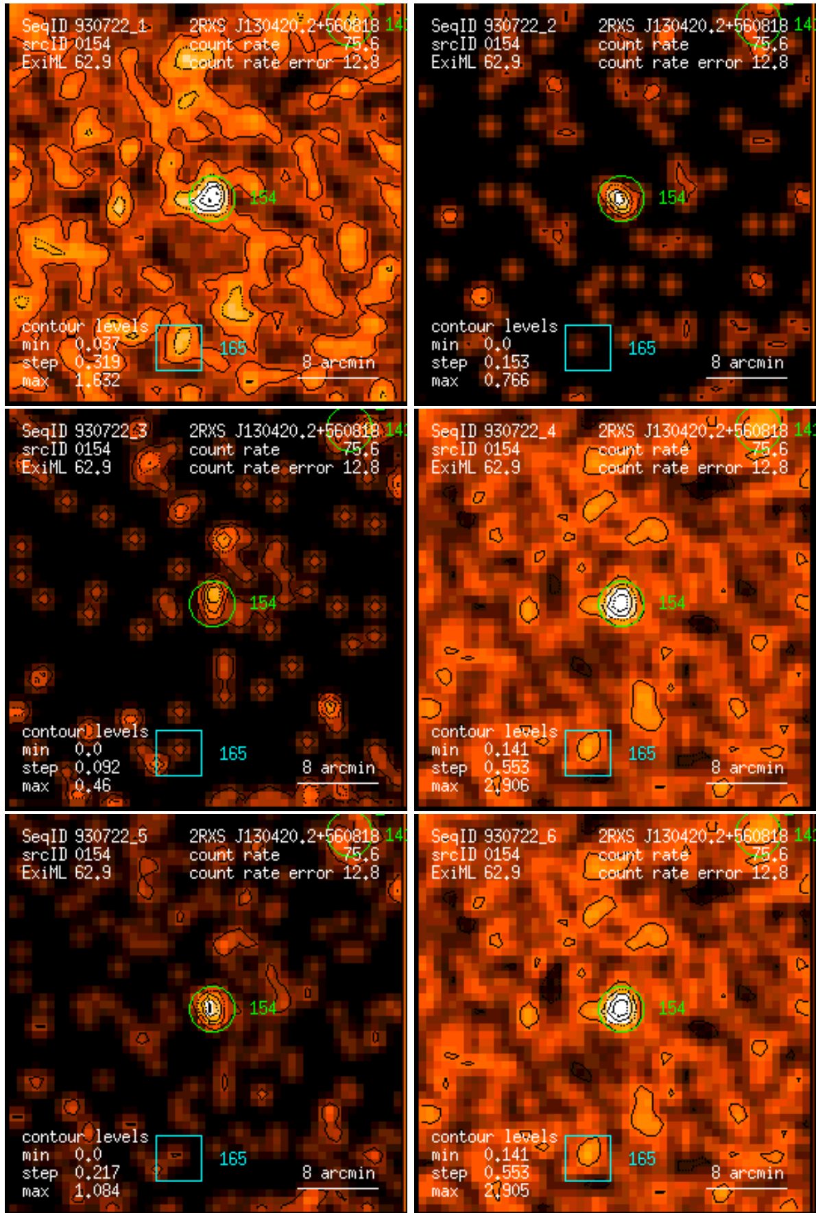
Figure 154: RASS 930722: detection 0154: band rate images, Gaussian filter: (1) PSPC channels 11 – 41, (2) 52 – 90, (3) 91 – 201, (4) 11 – 235, (5) 52 – 201, (6) 11 – 201. Broad band rates in counts/ks. Band rate contour levels in counts/ks/arcmin 2 .
