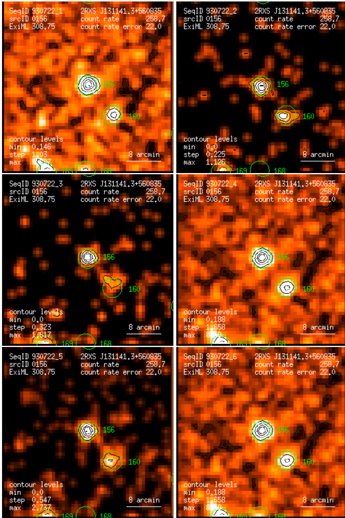
Figure 156: RASS 930722: detection 0156: band rate images, Gaussian filter: (1) PSPC channels 11 – 41, (2) 52 – 90, (3) 91 – 201, (4) 11 – 235, (5) 52 – 201, (6) 11 – 201. Broad band rates in counts/ks. Band rate contour levels in counts/ks/arcmin 2 .
