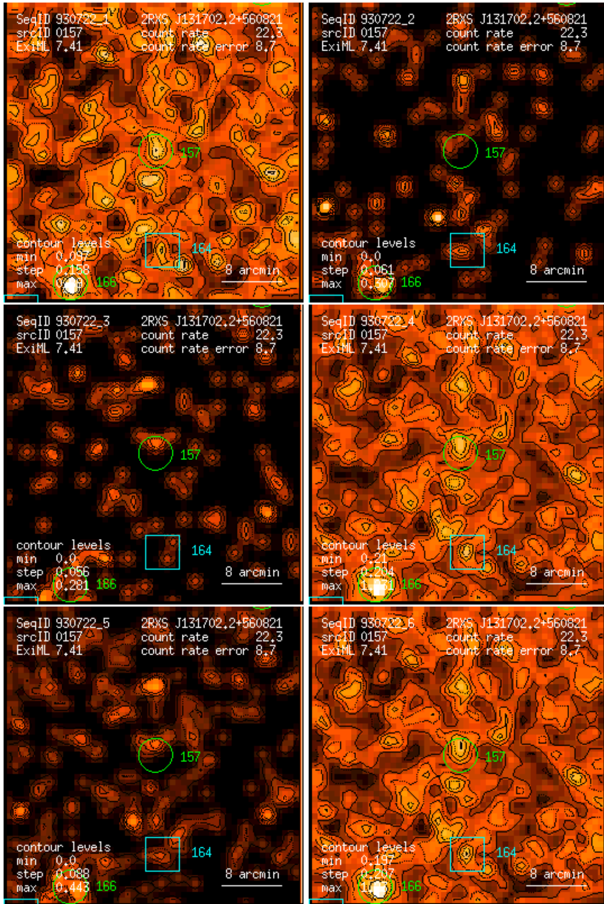
Figure 157: RASS 930722: detection 0157: band rate images, Gaussian filter: (1) PSPC channels 11 – 41, (2) 52 – 90, (3) 91 – 201, (4) 11 – 235, (5) 52 – 201, (6) 11 – 201. Broad band rates in counts/ks. Band rate contour levels in counts/ks/arcmin 2 .
