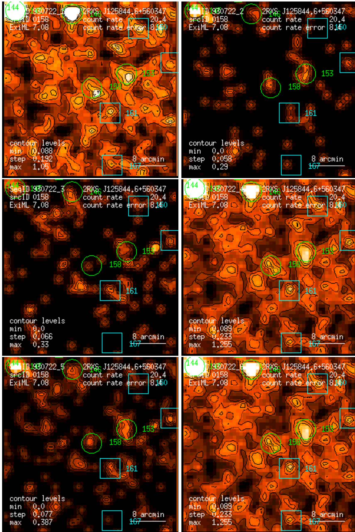
Figure 158: RASS 930722: detection 0158: band rate images, Gaussian filter: (1) PSPC channels 11 – 41, (2) 52 – 90, (3) 91 – 201, (4) 11 – 235, (5) 52 – 201, (6) 11 – 201. Broad band rates in counts/ks. Band rate contour levels in counts/ks/arcmin 2 .
