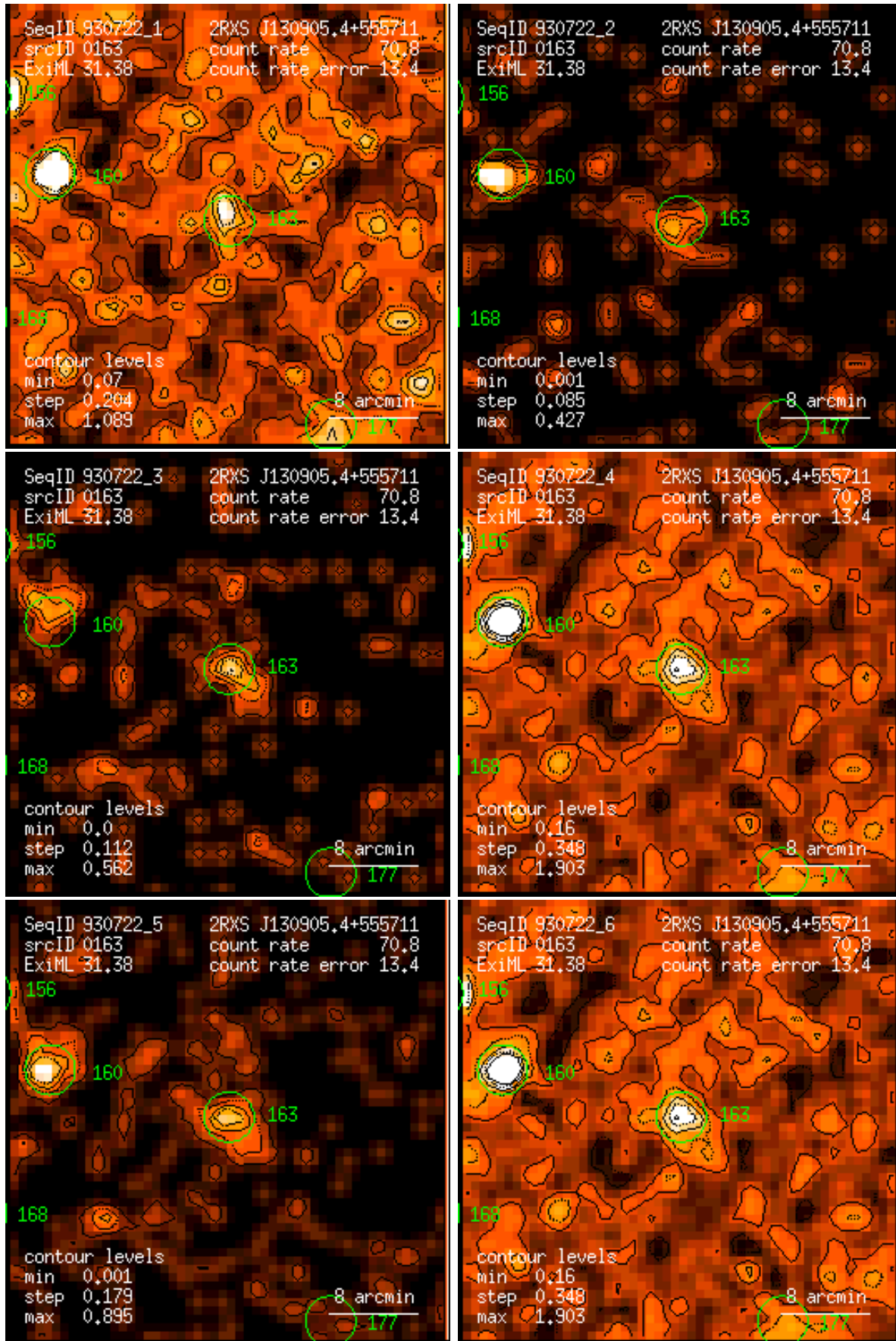
Figure 163: RASS 930722: detection 0163: band rate images, Gaussian filter: (1) PSPC channels 11 – 41, (2) 52 – 90, (3) 91 – 201, (4) 11 – 235, (5) 52 – 201, (6) 11 – 201. Broad band rates in counts/ks. Band rate contour levels in counts/ks/arcmin 2 .
